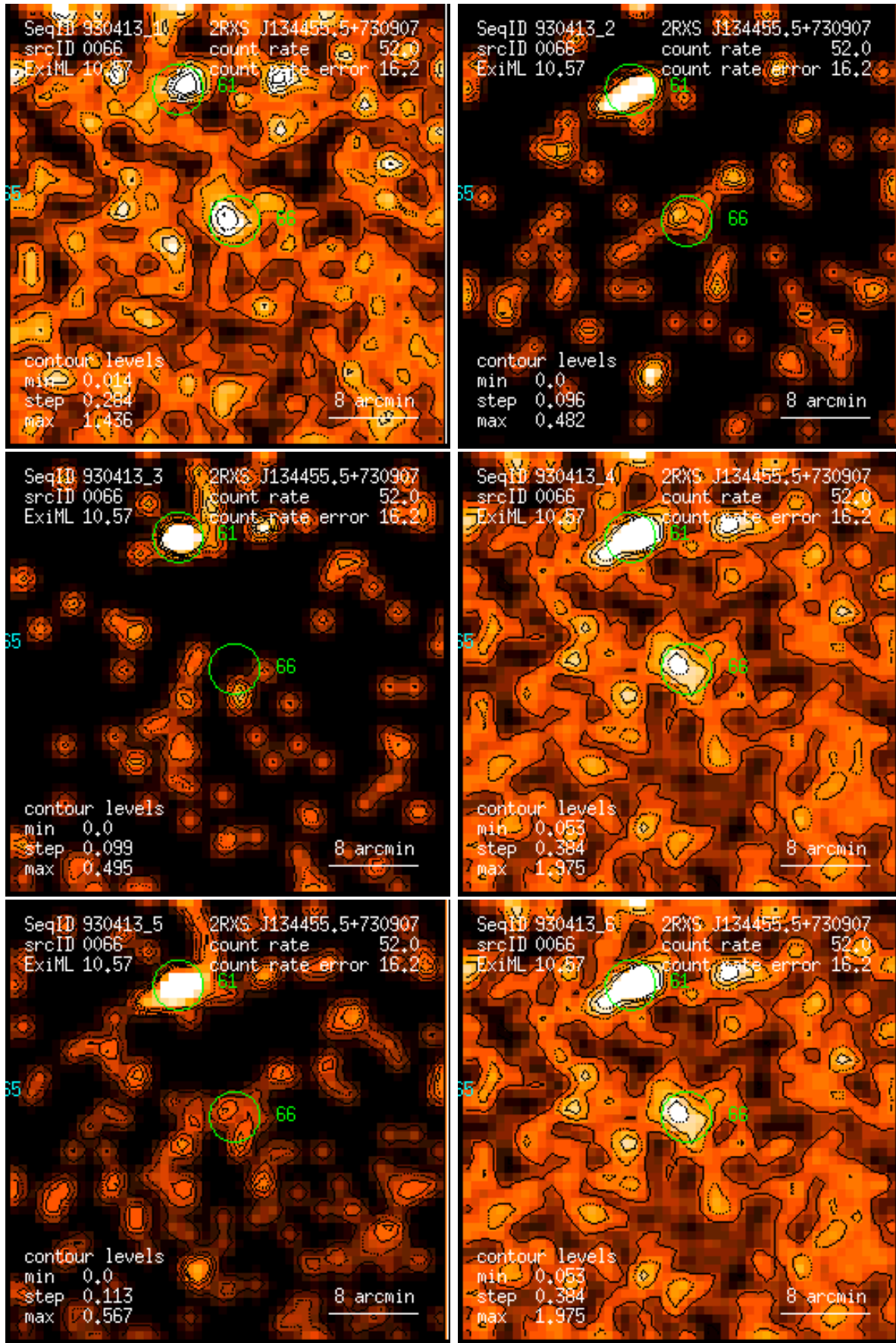
Figure 66: RASS 930413: detection 0066: band rate images, Gaussian filter: (1) PSPC channels 11 – 41, (2) 52 – 90, (3) 91 – 201, (4) 11 – 235, (5) 52 – 201, (6) 11 – 201. Broad band rates in counts/ks. Band rate contour levels in counts/ks/arcmin 2 .
