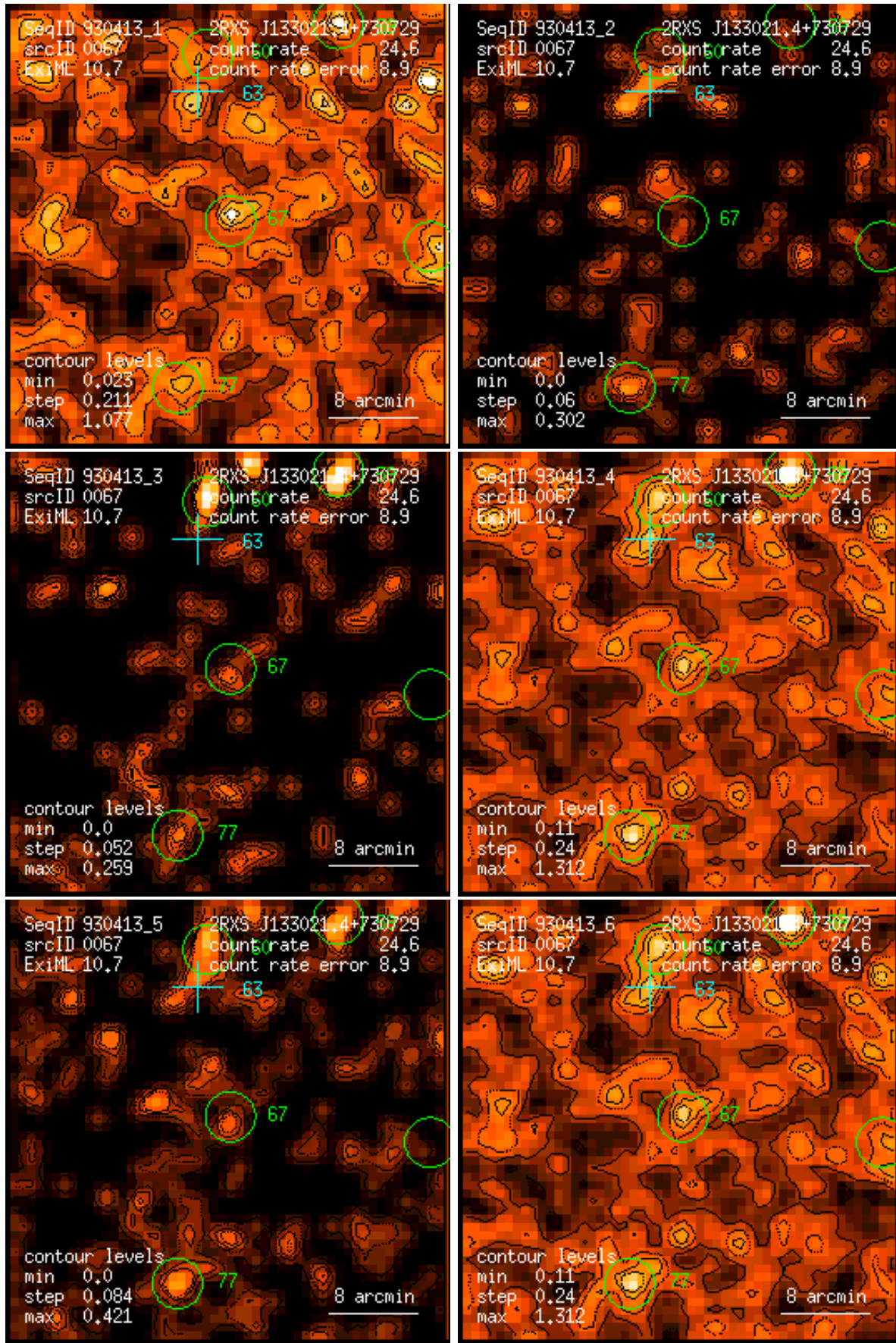
Figure 67: RASS 930413: detection 0067: band rate images, Gaussian filter: (1) PSPC channels 11 – 41, (2) 52 – 90, (3) 91 – 201, (4) 11 – 235, (5) 52 – 201, (6) 11 – 201. Broad band rates in counts/ks. Band rate contour levels in counts/ks/arcmin 2 .
