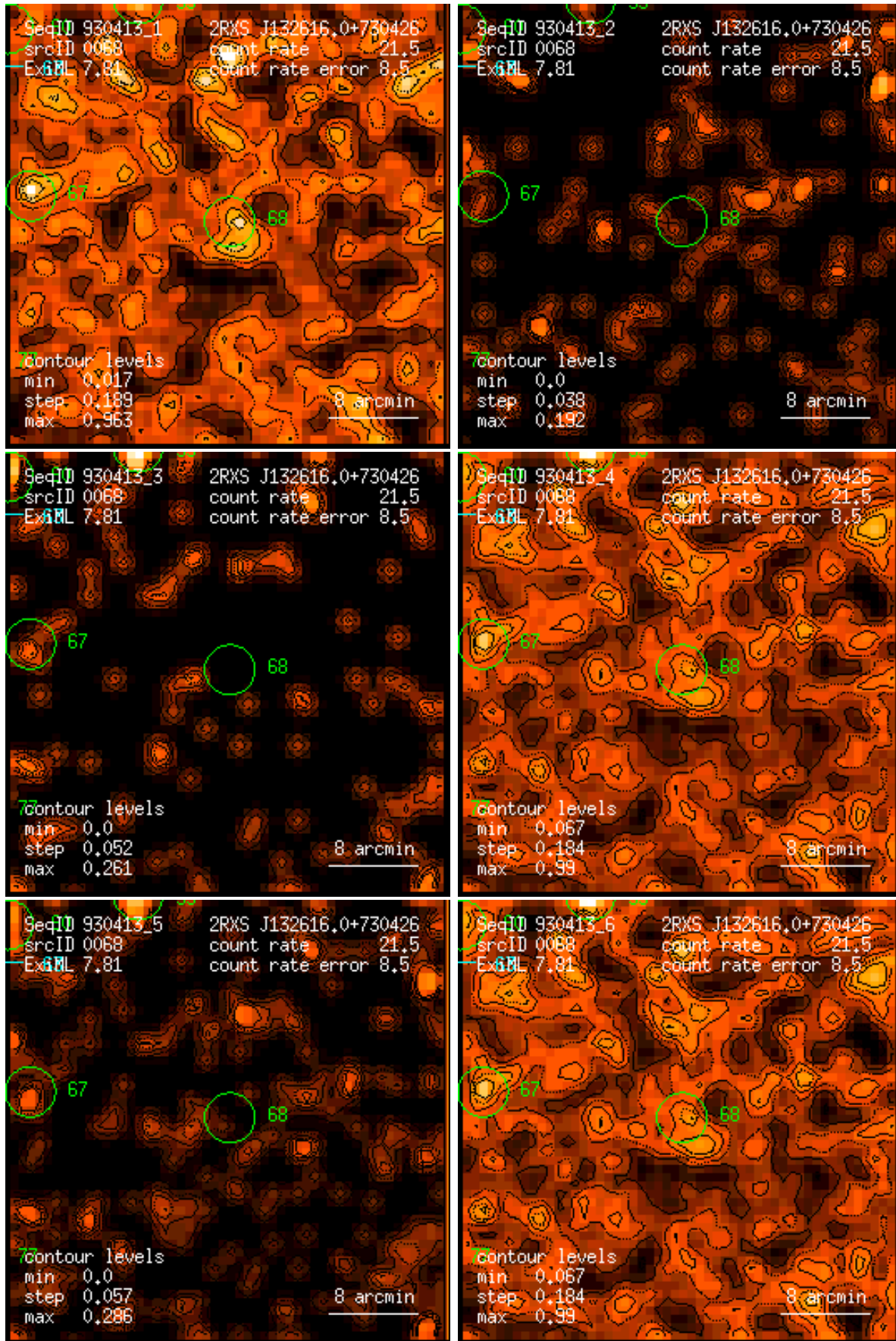
Figure 68: RASS 930413: detection 0068: band rate images, Gaussian filter: (1) PSPC channels 11 – 41, (2) 52 – 90, (3) 91 – 201, (4) 11 – 235, (5) 52 – 201, (6) 11 – 201. Broad band rates in counts/ks. Band rate contour levels in counts/ks/arcmin 2 .
