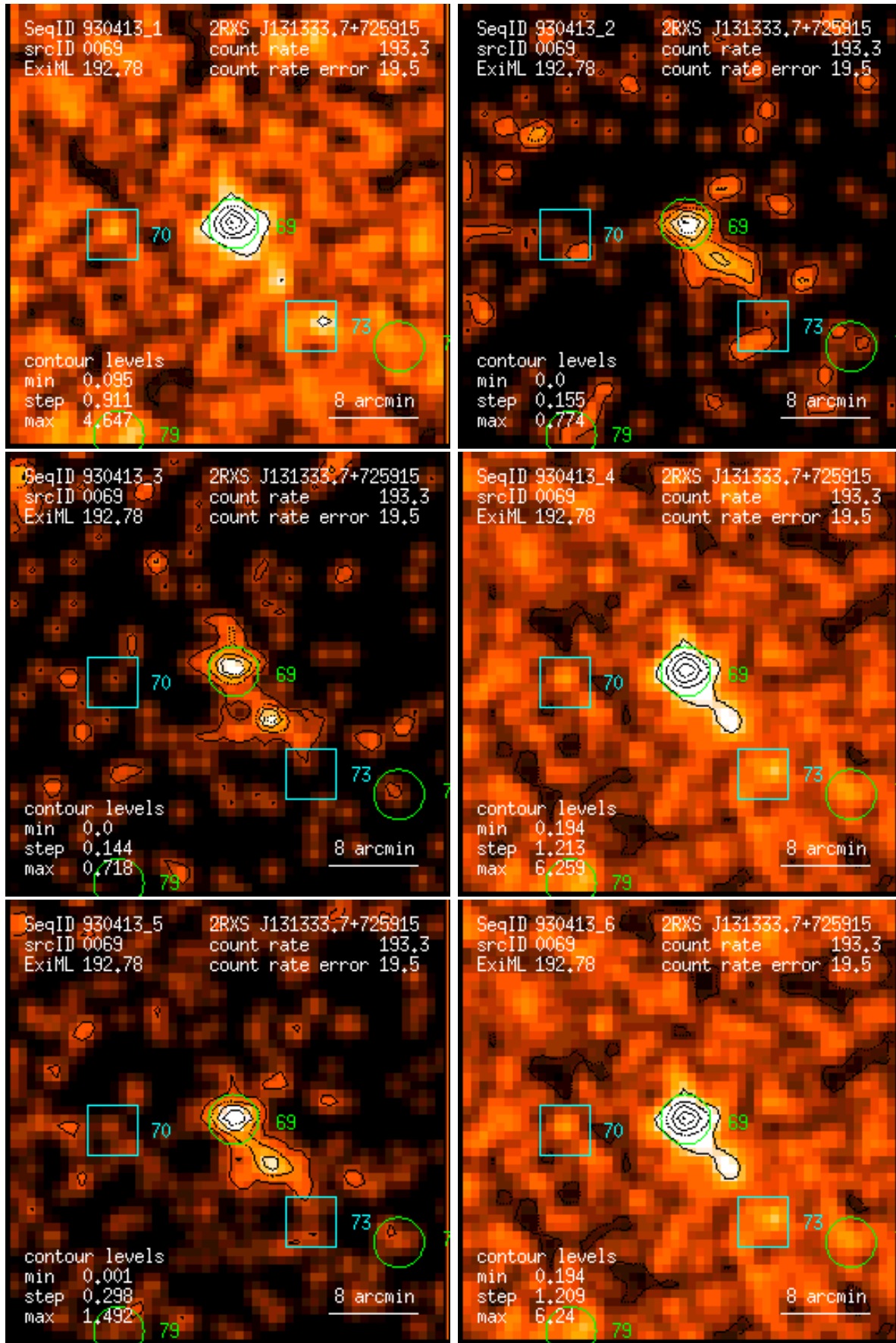
Figure 69: RASS 930413: detection 0069: band rate images, Gaussian filter: (1) PSPC channels 11 – 41, (2) 52 – 90, (3) 91 – 201, (4) 11 – 235, (5) 52 – 201, (6) 11 – 201. Broad band rates in counts/ks. Band rate contour levels in counts/ks/arcmin 2 .
