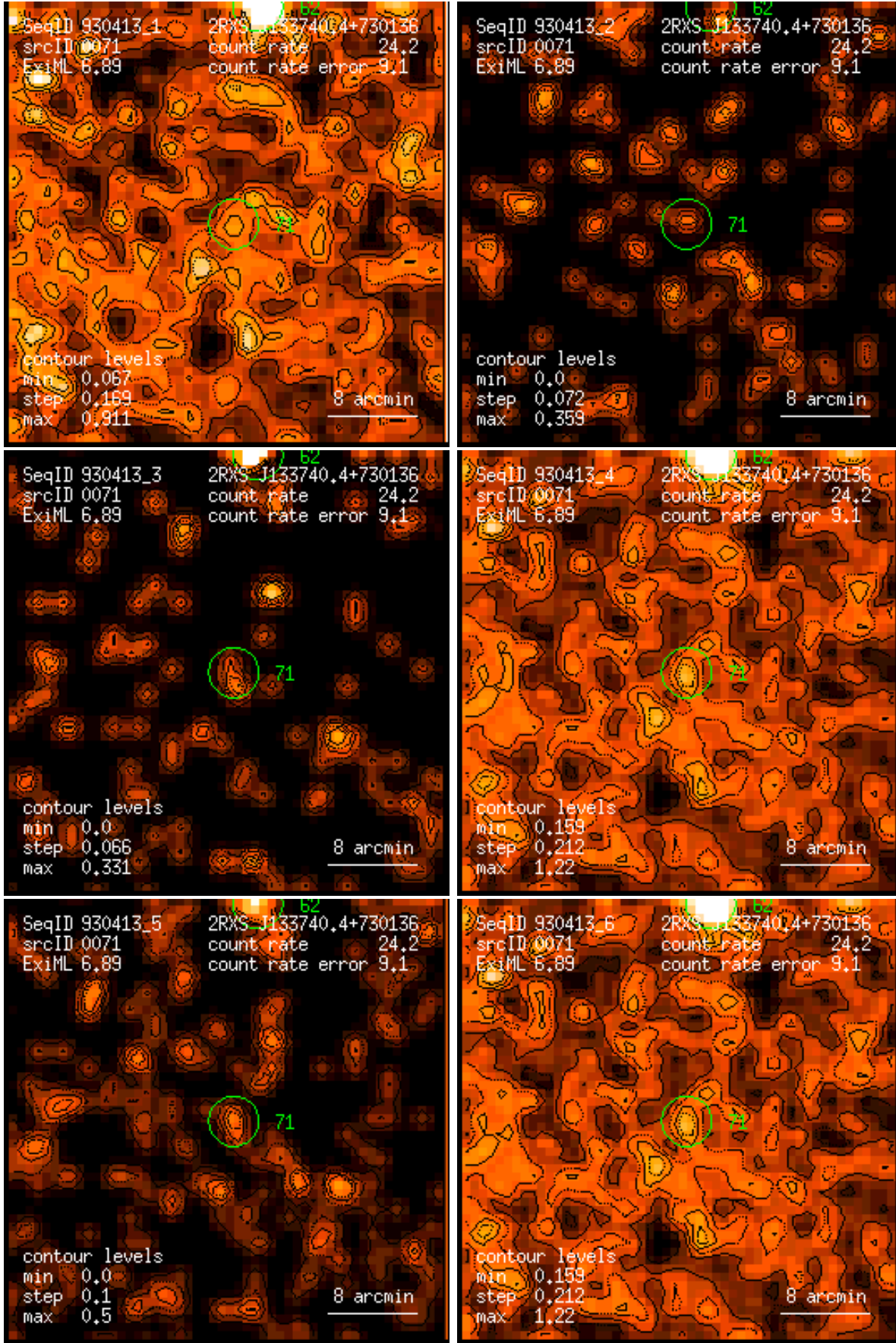
Figure 71: RASS 930413: detection 0071: band rate images, Gaussian filter: (1) PSPC channels 11 – 41, (2) 52 – 90, (3) 91 – 201, (4) 11 – 235, (5) 52 – 201, (6) 11 – 201. Broad band rates in counts/ks. Band rate contour levels in counts/ks/arcmin 2 .
