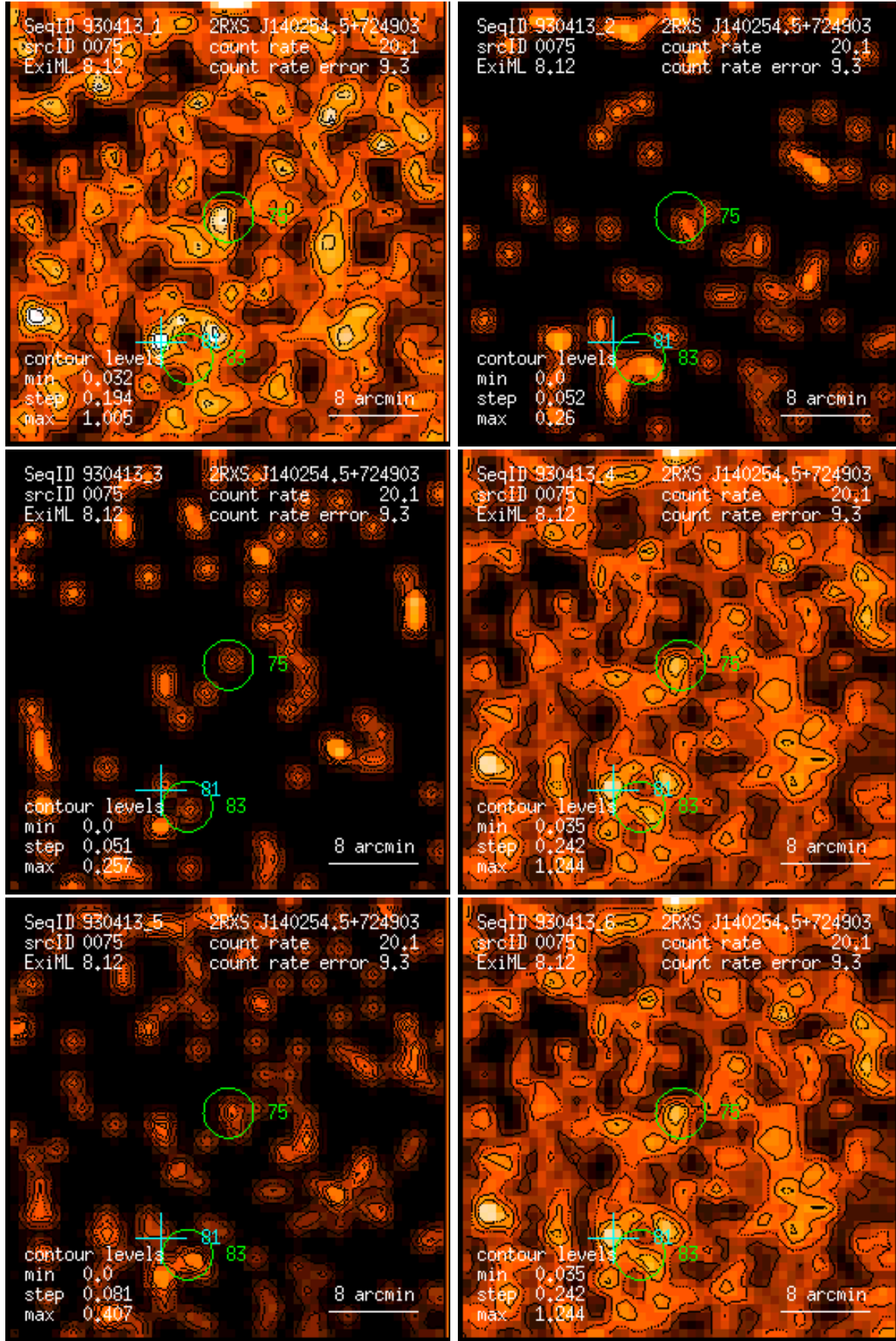
Figure 75: RASS 930413: detection 0075: band rate images, Gaussian filter: (1) PSPC channels 11 – 41, (2) 52 – 90, (3) 91 – 201, (4) 11 – 235, (5) 52 – 201, (6) 11 – 201. Broad band rates in counts/ks. Band rate contour levels in counts/ks/arcmin 2 .
