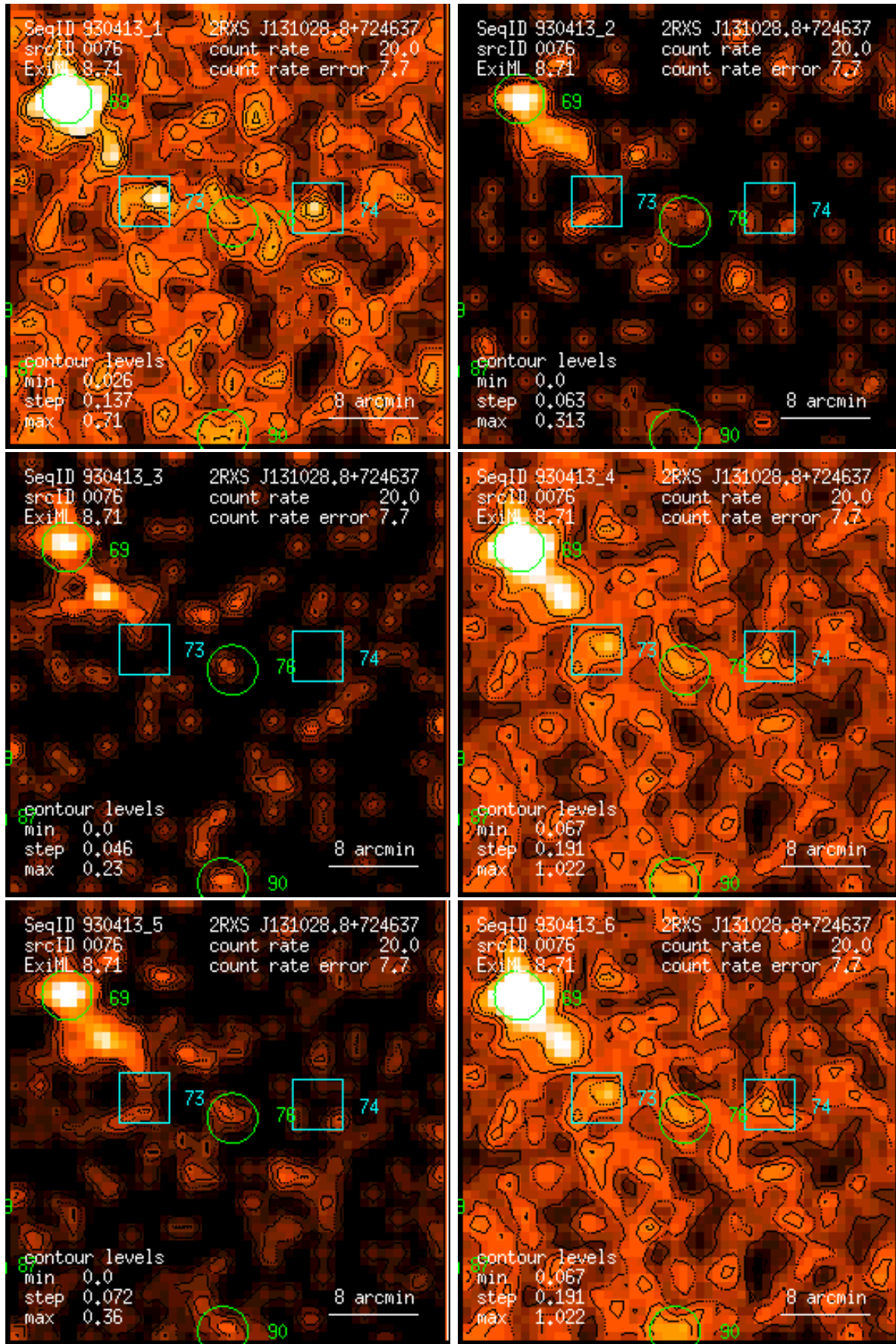
Figure 76: RASS 930413: detection 0076: band rate images, Gaussian filter: (1) PSPC channels 11 – 41, (2) 52 – 90, (3) 91 – 201, (4) 11 – 235, (5) 52 – 201, (6) 11 – 201. Broad band rates in counts/ks. Band rate contour levels in counts/ks/arcmin 2 .
