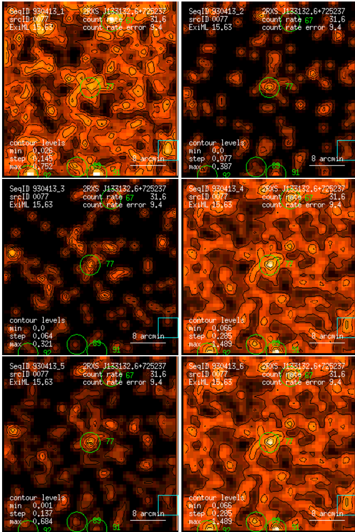
Figure 77: RASS 930413: detection 0077: band rate images, Gaussian filter: (1) PSPC channels 11 – 41, (2) 52 – 90, (3) 91 – 201, (4) 11 – 235, (5) 52 – 201, (6) 11 – 201. Broad band rates in counts/ks. Band rate contour levels in counts/ks/arcmin 2 .
