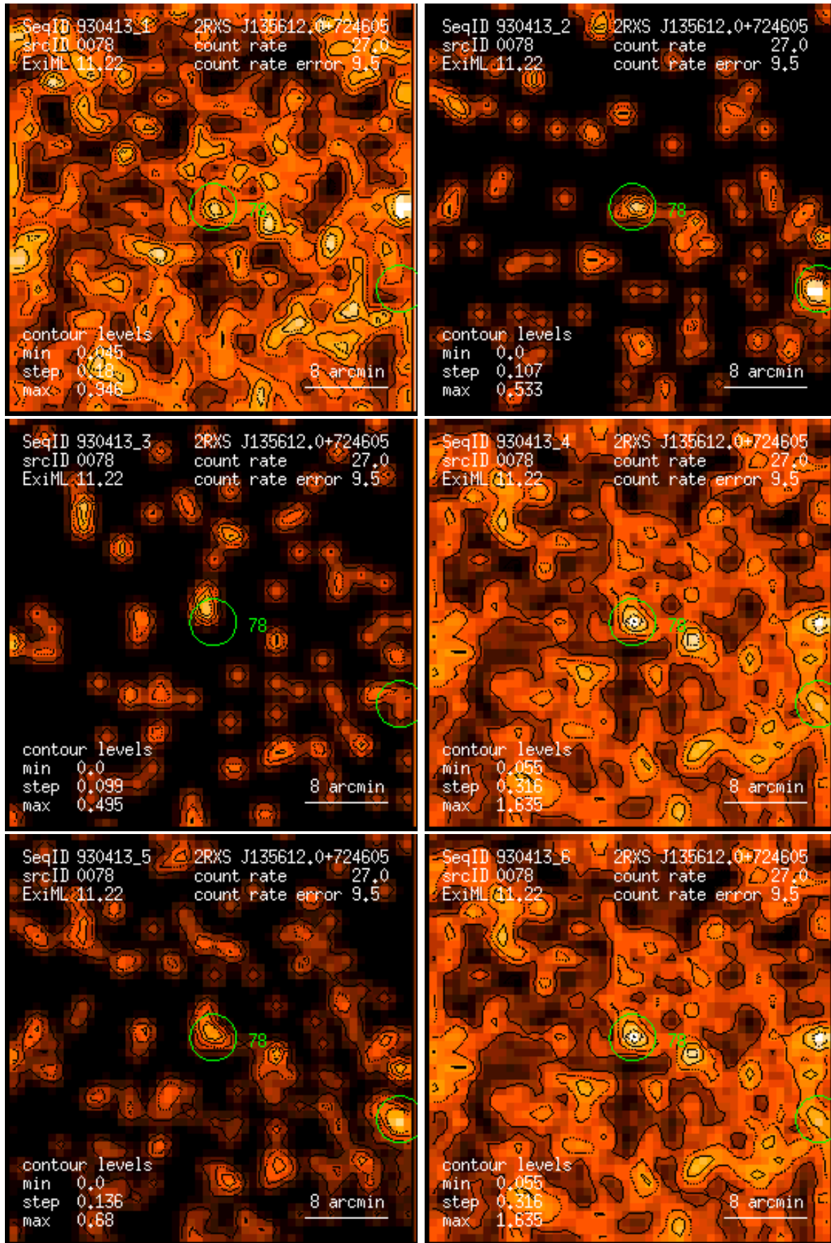
Figure 78: RASS 930413: detection 0078: band rate images, Gaussian filter: (1) PSPC channels 11 – 41, (2) 52 – 90, (3) 91 – 201, (4) 11 – 235, (5) 52 – 201, (6) 11 – 201. Broad band rates in counts/ks. Band rate contour levels in counts/ks/arcmin 2 .
