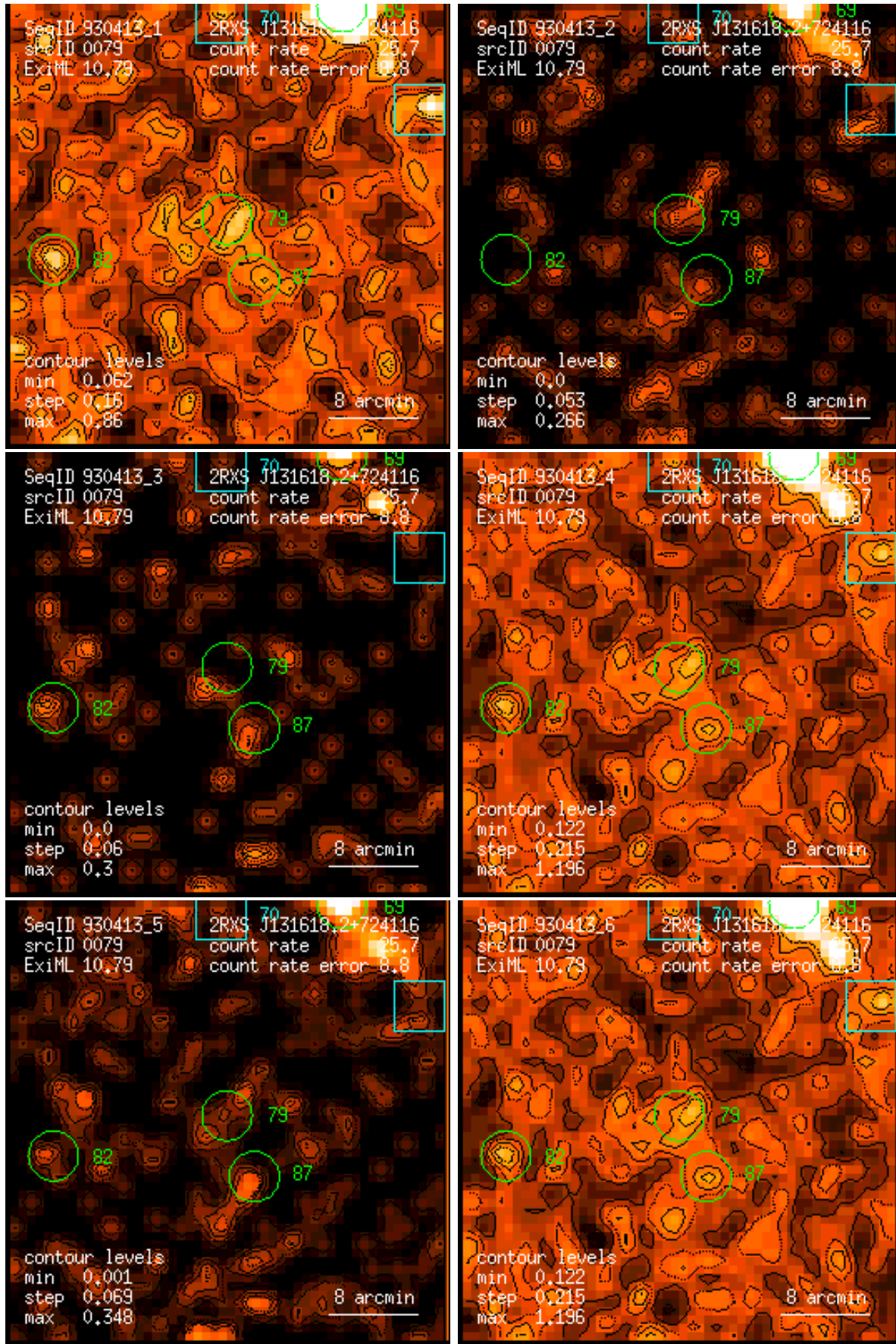
Figure 79: RASS 930413: detection 0079: band rate images, Gaussian filter: (1) PSPC channels 11 – 41, (2) 52 – 90, (3) 91 – 201, (4) 11 – 235, (5) 52 – 201, (6) 11 – 201. Broad band rates in counts/ks. Band rate contour levels in counts/ks/arcmin 2 .
