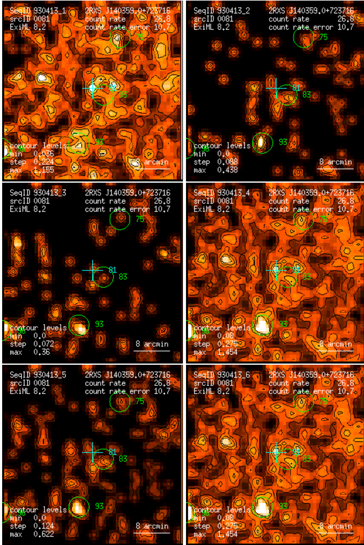
Figure 81: RASS 930413: detection 0081: band rate images, Gaussian filter: (1) PSPC channels 11 – 41, (2) 52 – 90, (3) 91 – 201, (4) 11 – 235, (5) 52 – 201, (6) 11 – 201. Broad band rates in counts/ks. Band rate contour levels in counts/ks/arcmin 2 .
