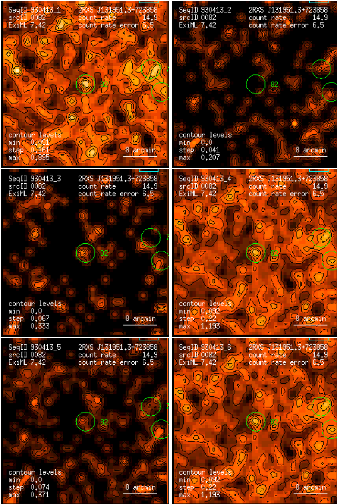
Figure 82: RASS 930413: detection 0082: band rate images, Gaussian filter: (1) PSPC channels 11 – 41, (2) 52 – 90, (3) 91 – 201, (4) 11 – 235, (5) 52 – 201, (6) 11 – 201. Broad band rates in counts/ks. Band rate contour levels in counts/ks/arcmin 2 .
