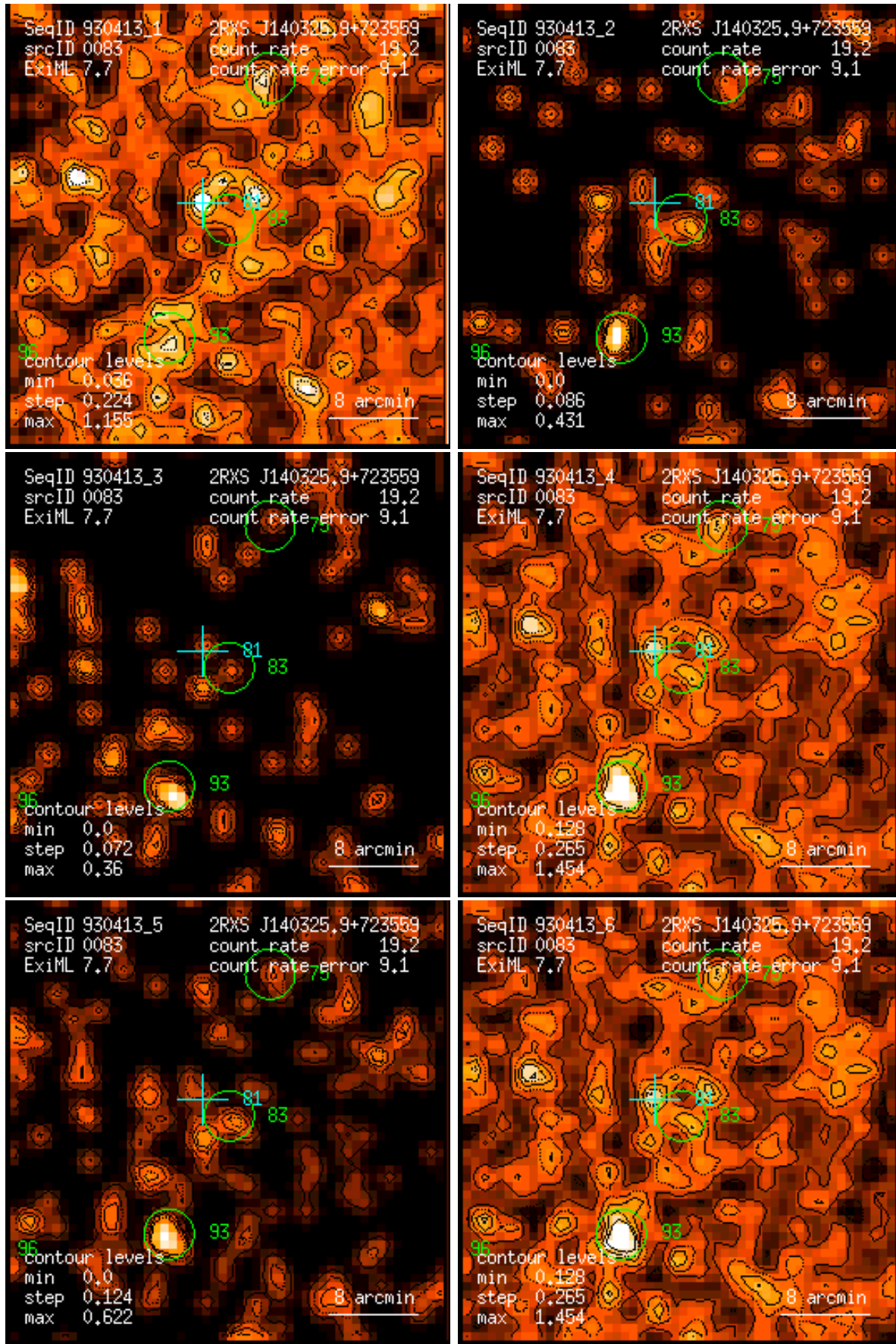
Figure 83: RASS 930413: detection 0083: band rate images, Gaussian filter: (1) PSPC channels 11 – 41, (2) 52 – 90, (3) 91 – 201, (4) 11 – 235, (5) 52 – 201, (6) 11 – 201. Broad band rates in counts/ks. Band rate contour levels in counts/ks/arcmin 2 .
