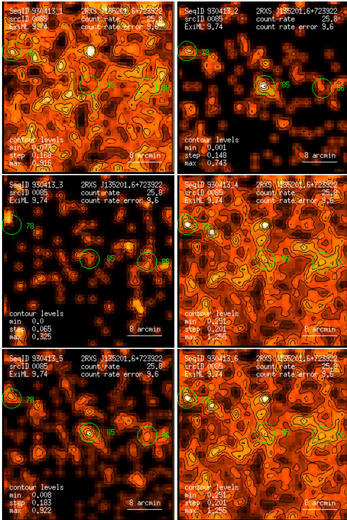
Figure 85: RASS 930413: detection 0085: band rate images, Gaussian filter: (1) PSPC channels 11 – 41, (2) 52 – 90, (3) 91 – 201, (4) 11 – 235, (5) 52 – 201, (6) 11 – 201. Broad band rates in counts/ks. Band rate contour levels in counts/ks/arcmin 2 .
