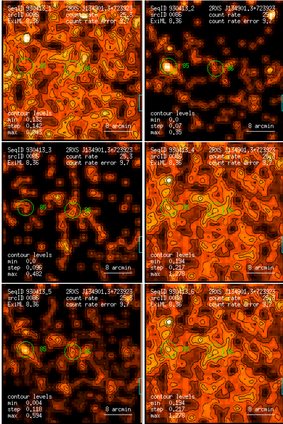
Figure 86: RASS 930413: detection 0086: band rate images, Gaussian filter: (1) PSPC channels 11 – 41, (2) 52 – 90, (3) 91 – 201, (4) 11 – 235, (5) 52 – 201, (6) 11 – 201. Broad band rates in counts/ks. Band rate contour levels in counts/ks/arcmin 2 .
