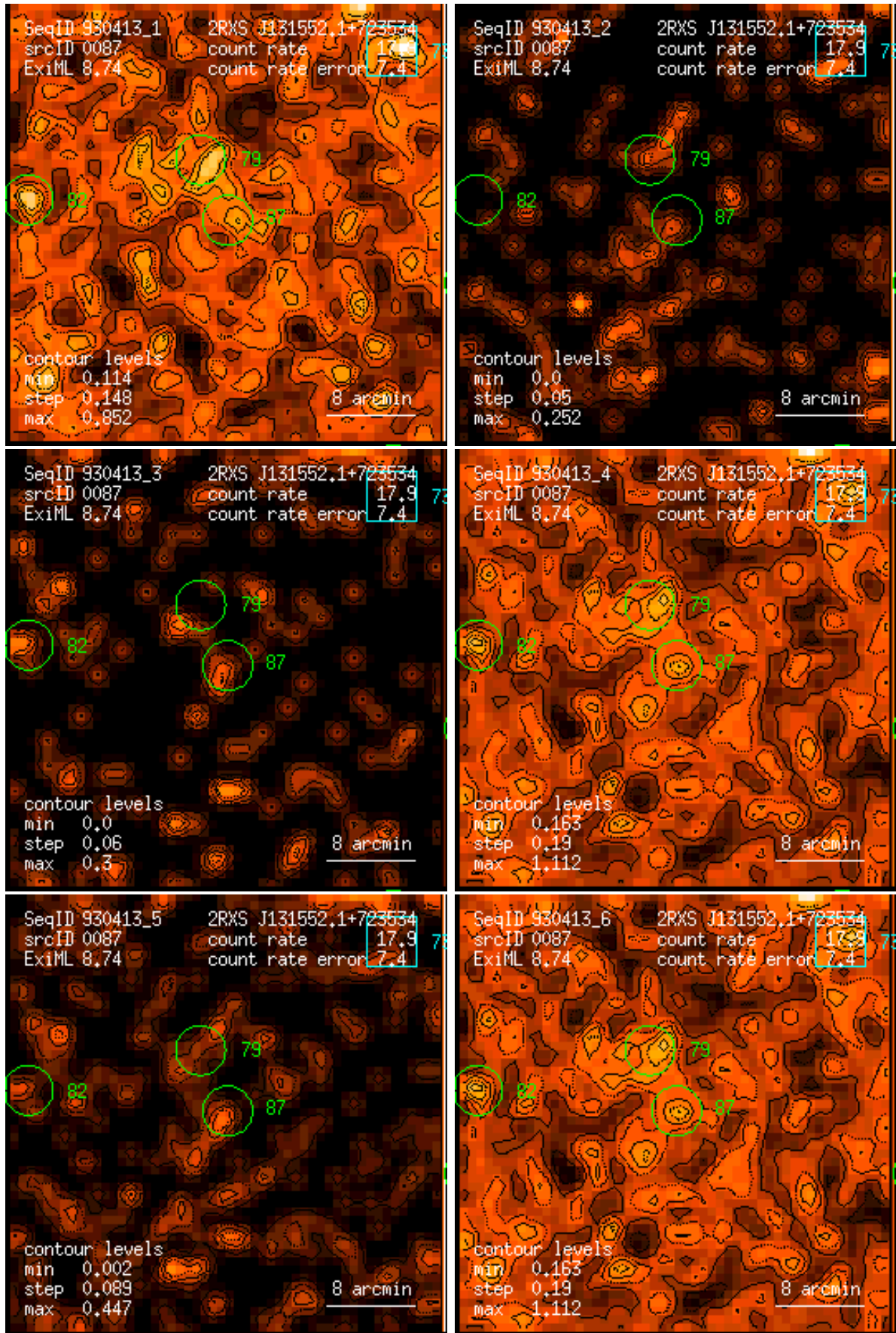
Figure 87: RASS 930413: detection 0087: band rate images, Gaussian filter: (1) PSPC channels 11 – 41, (2) 52 – 90, (3) 91 – 201, (4) 11 – 235, (5) 52 – 201, (6) 11 – 201. Broad band rates in counts/ks. Band rate contour levels in counts/ks/arcmin 2 .
