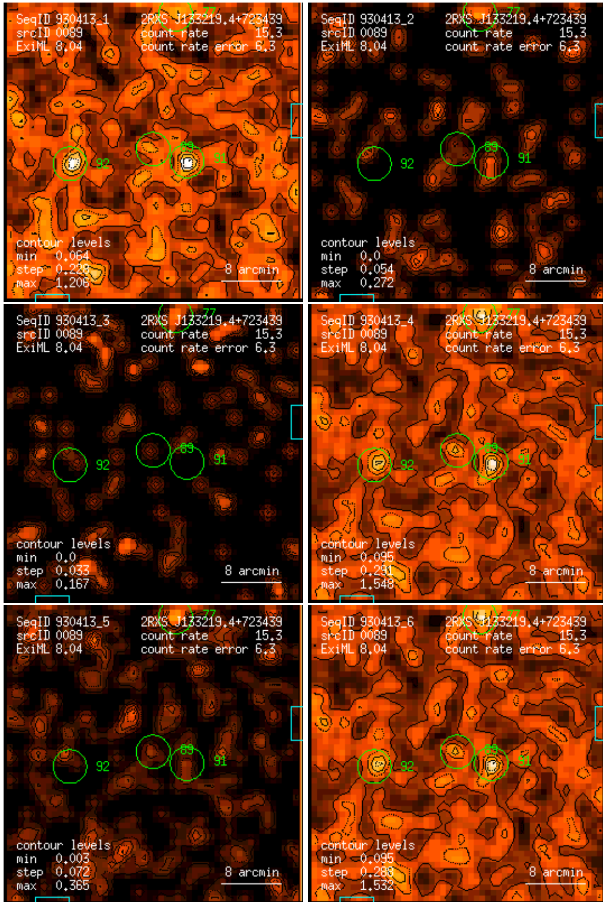
Figure 89: RASS 930413: detection 0089: band rate images, Gaussian filter: (1) PSPC channels 11 – 41, (2) 52 – 90, (3) 91 – 201, (4) 11 – 235, (5) 52 – 201, (6) 11 – 201. Broad band rates in counts/ks. Band rate contour levels in counts/ks/arcmin 2 .
