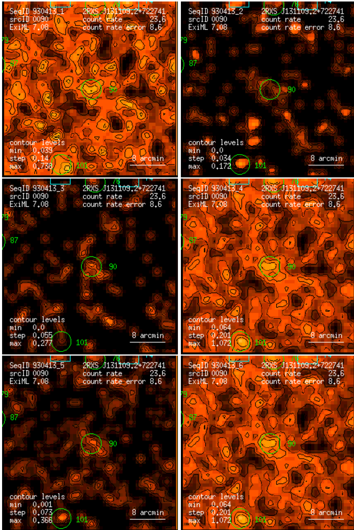
Figure 90: RASS 930413: detection 0090: band rate images, Gaussian filter: (1) PSPC channels 11 – 41, (2) 52 – 90, (3) 91 – 201, (4) 11 – 235, (5) 52 – 201, (6) 11 – 201. Broad band rates in counts/ks. Band rate contour levels in counts/ks/arcmin 2 .
