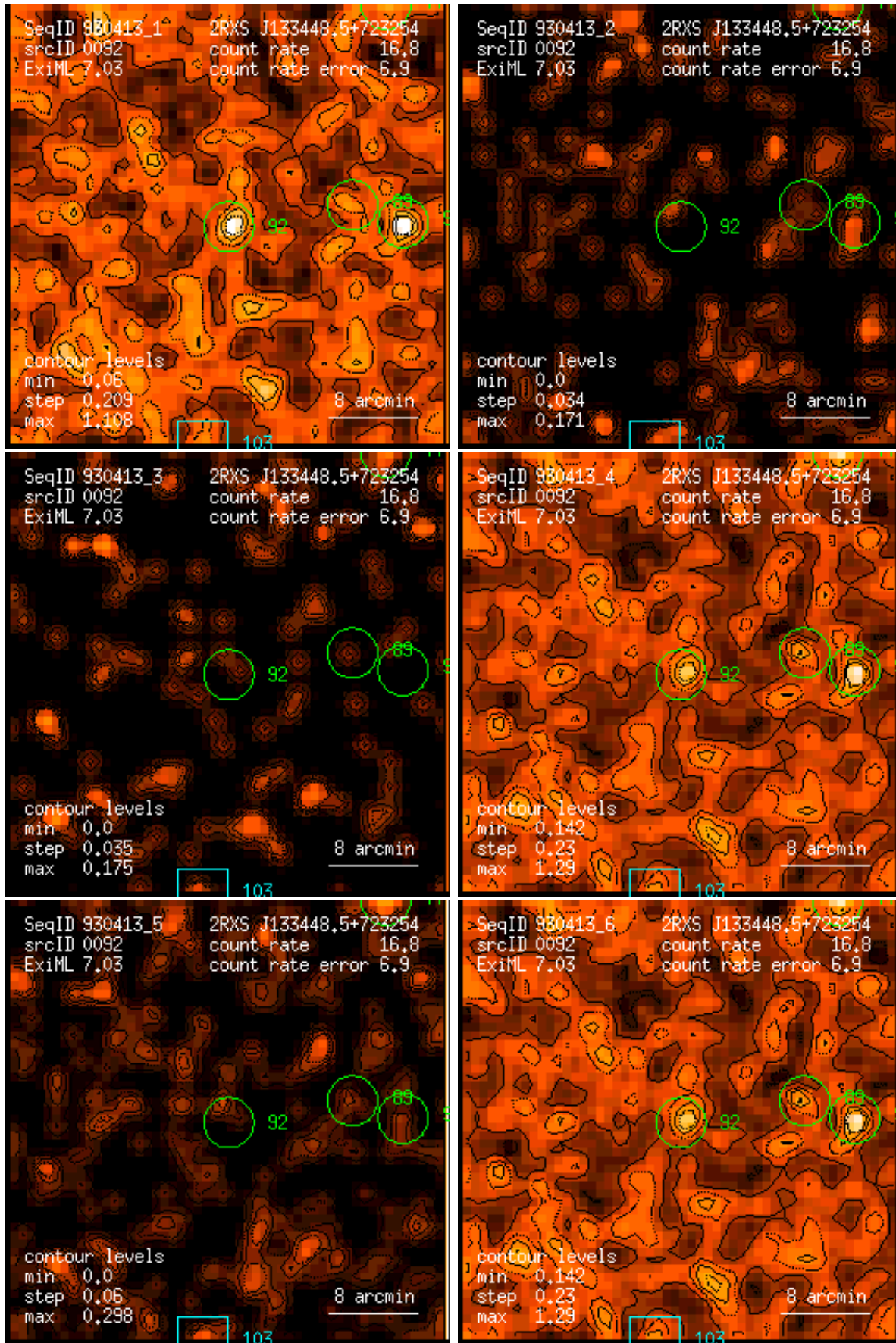
Figure 92: RASS 930413: detection 0092: band rate images, Gaussian filter: (1) PSPC channels 11 – 41, (2) 52 – 90, (3) 91 – 201, (4) 11 – 235, (5) 52 – 201, (6) 11 – 201. Broad band rates in counts/ks. Band rate contour levels in counts/ks/arcmin 2 .
