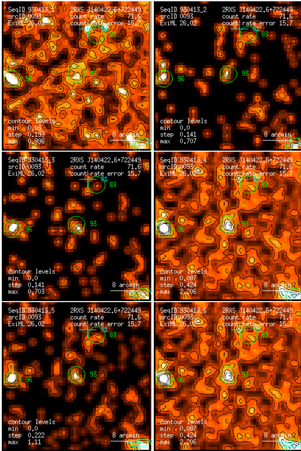
Figure 93: RASS 930413: detection 0093: band rate images, Gaussian filter: (1) PSPC channels 11 – 41, (2) 52 – 90, (3) 91 – 201, (4) 11 – 235, (5) 52 – 201, (6) 11 – 201. Broad band rates in counts/ks. Band rate contour levels in counts/ks/arcmin 2 .
