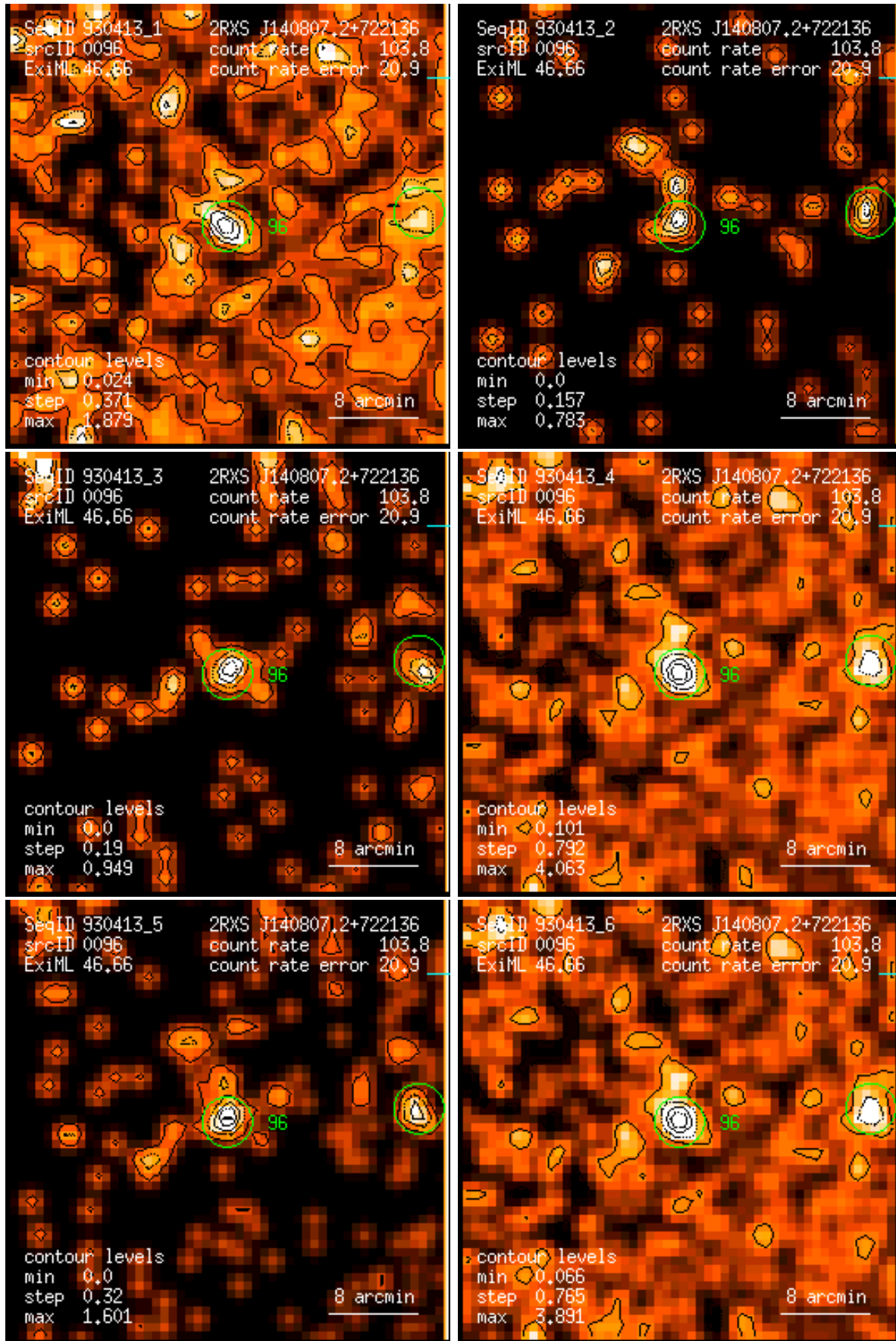
Figure 96: RASS 930413: detection 0096: band rate images, Gaussian filter: (1) PSPC channels 11 – 41, (2) 52 – 90, (3) 91 – 201, (4) 11 – 235, (5) 52 – 201, (6) 11 – 201. Broad band rates in counts/ks. Band rate contour levels in counts/ks/arcmin 2 .
