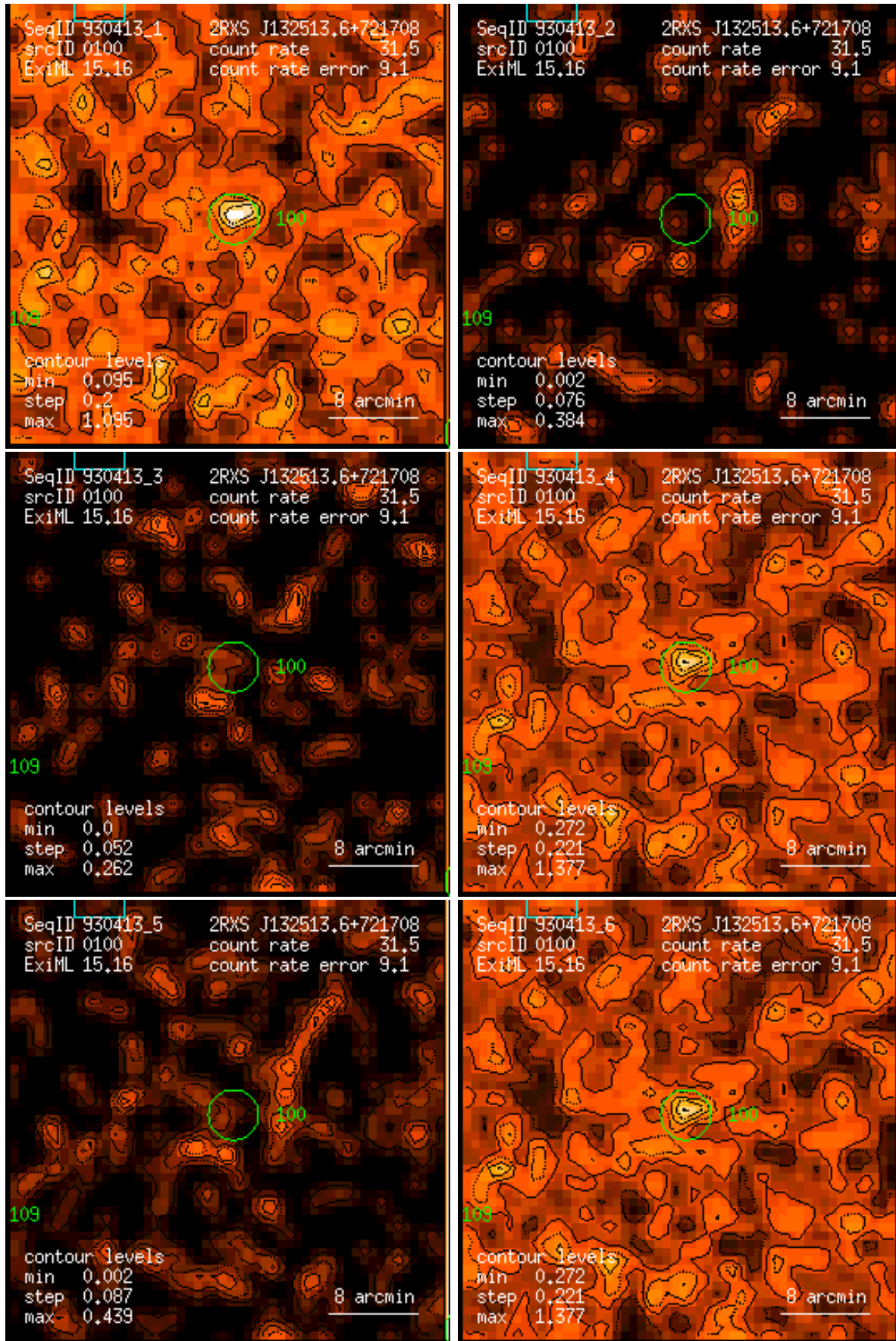
Figure 100: RASS 930413: detection 0100: band rate images, Gaussian filter: (1) PSPC channels 11 – 41, (2) 52 – 90, (3) 91 – 201, (4) 11 – 235, (5) 52 – 201, (6) 11 – 201. Broad band rates in counts/ks. Band rate contour levels in counts/ks/arcmin 2 .
