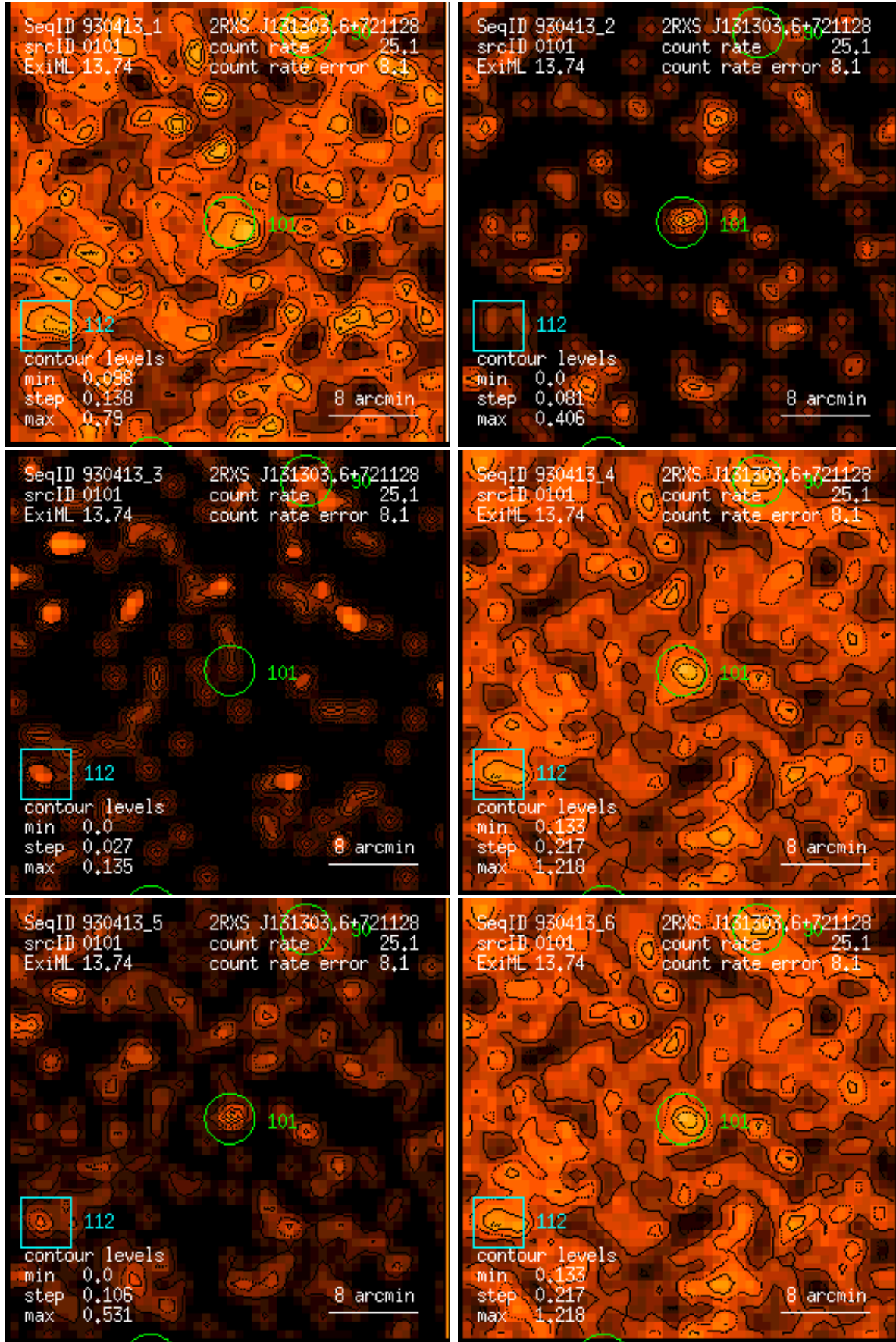
Figure 101: RASS 930413: detection 0101: band rate images, Gaussian filter: (1) PSPC channels 11 – 41, (2) 52 – 90, (3) 91 – 201, (4) 11 – 235, (5) 52 – 201, (6) 11 – 201. Broad band rates in counts/ks. Band rate contour levels in counts/ks/arcmin 2 .
