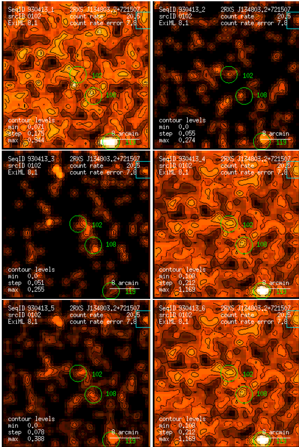
Figure 102: RASS 930413: detection 0102: band rate images, Gaussian filter: (1) PSPC channels 11 – 41, (2) 52 – 90, (3) 91 – 201, (4) 11 – 235, (5) 52 – 201, (6) 11 – 201. Broad band rates in counts/ks. Band rate contour levels in counts/ks/arcmin 2 .
