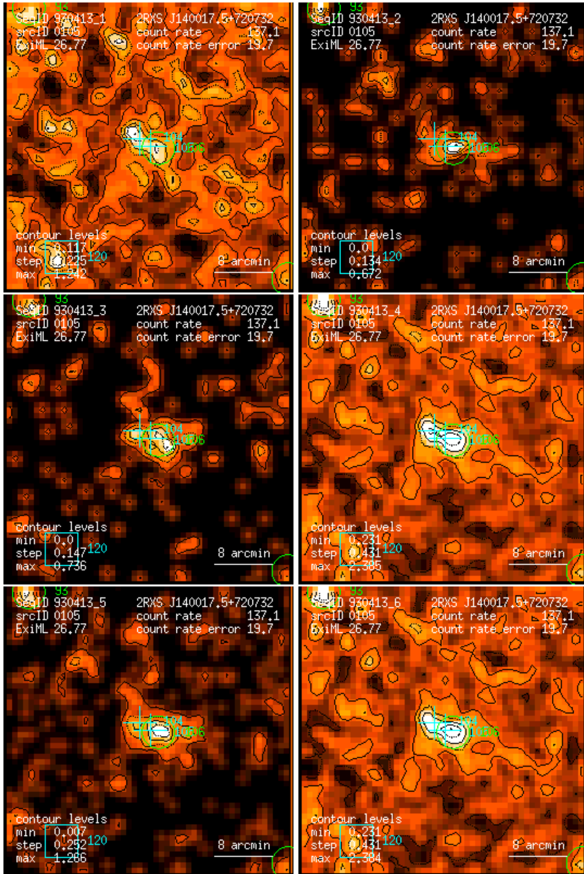
Figure 105: RASS 930413: detection 0105: band rate images, Gaussian filter: (1) PSPC channels 11 – 41, (2) 52 – 90, (3) 91 – 201, (4) 11 – 235, (5) 52 – 201, (6) 11 – 201. Broad band rates in counts/ks. Band rate contour levels in counts/ks/arcmin 2 .
