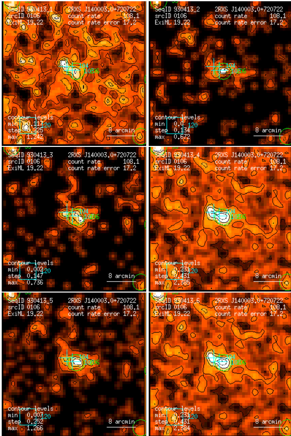
Figure 106: RASS 930413: detection 0106: band rate images, Gaussian filter: (1) PSPC channels 11 – 41, (2) 52 – 90, (3) 91 – 201, (4) 11 – 235, (5) 52 – 201, (6) 11 – 201. Broad band rates in counts/ks. Band rate contour levels in counts/ks/arcmin 2 .
