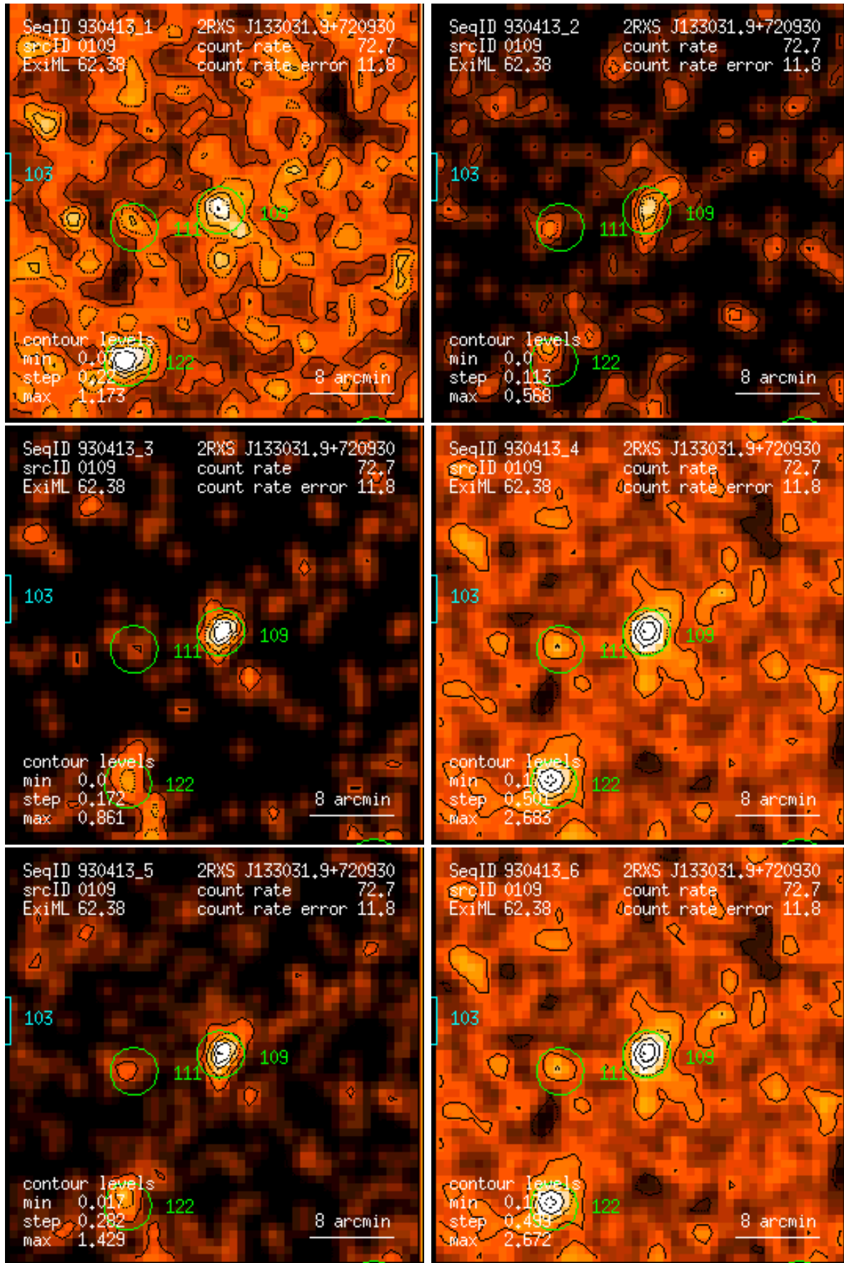
Figure 109: RASS 930413: detection 0109: band rate images, Gaussian filter: (1) PSPC channels 11 – 41, (2) 52 – 90, (3) 91 – 201, (4) 11 – 235, (5) 52 – 201, (6) 11 – 201. Broad band rates in counts/ks. Band rate contour levels in counts/ks/arcmin 2 .
