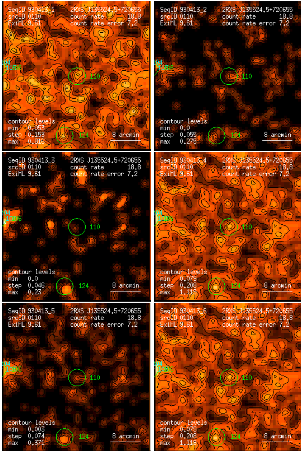
Figure 110: RASS 930413: detection 0110: band rate images, Gaussian filter: (1) PSPC channels 11 – 41, (2) 52 – 90, (3) 91 – 201, (4) 11 – 235, (5) 52 – 201, (6) 11 – 201. Broad band rates in counts/ks. Band rate contour levels in counts/ks/arcmin 2 .
