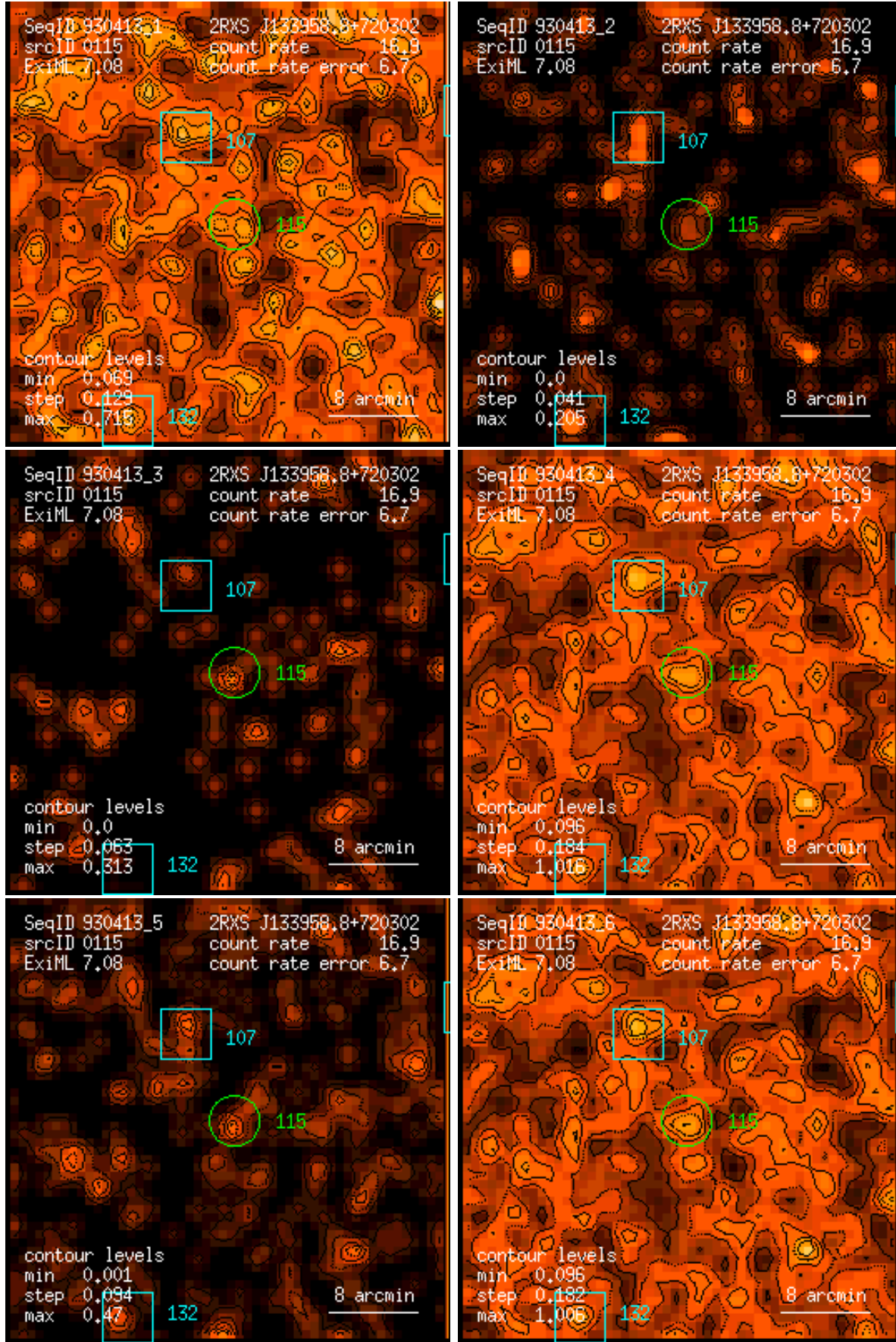
Figure 115: RASS 930413: detection 0115: band rate images, Gaussian filter: (1) PSPC channels 11 – 41, (2) 52 – 90, (3) 91 – 201, (4) 11 – 235, (5) 52 – 201, (6) 11 – 201. Broad band rates in counts/ks. Band rate contour levels in counts/ks/arcmin 2 .
