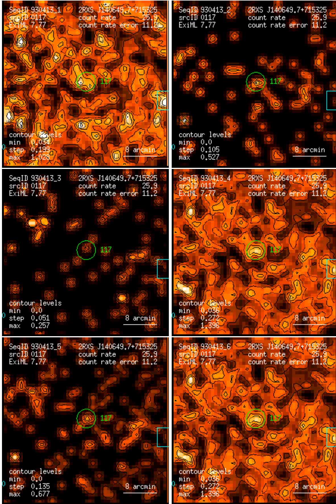
Figure 117: RASS 930413: detection 0117: band rate images, Gaussian filter: (1) PSPC channels 11 – 41, (2) 52 – 90, (3) 91 – 201, (4) 11 – 235, (5) 52 – 201, (6) 11 – 201. Broad band rates in counts/ks. Band rate contour levels in counts/ks/arcmin 2 .
