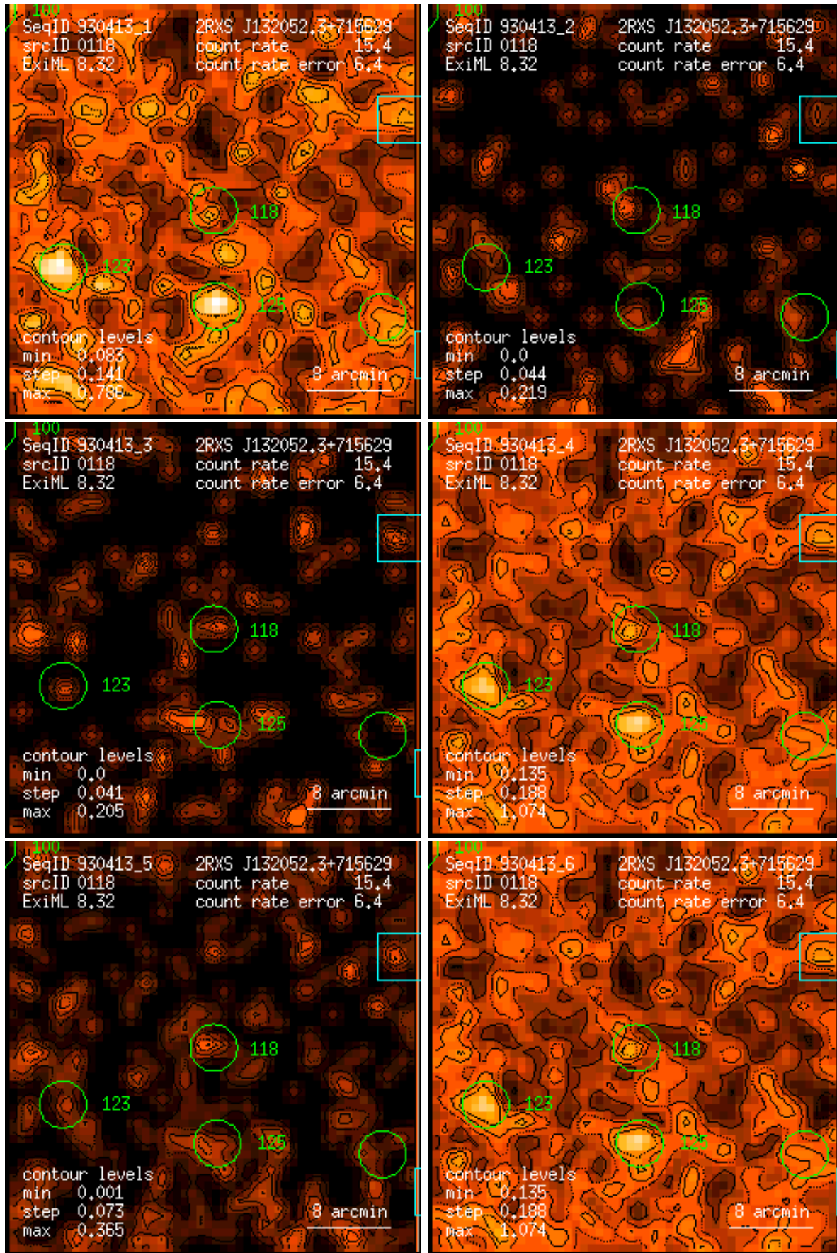
Figure 118: RASS 930413: detection 0118: band rate images, Gaussian filter: (1) PSPC channels 11 – 41, (2) 52 – 90, (3) 91 – 201, (4) 11 – 235, (5) 52 – 201, (6) 11 – 201. Broad band rates in counts/ks. Band rate contour levels in counts/ks/arcmin 2 .
