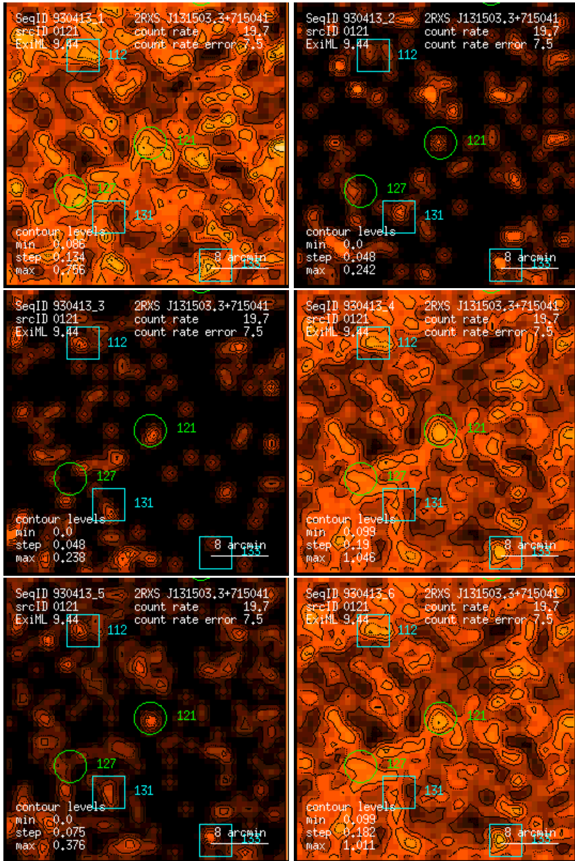
Figure 121: RASS 930413: detection 0121: band rate images, Gaussian filter: (1) PSPC channels 11 – 41, (2) 52 – 90, (3) 91 – 201, (4) 11 – 235, (5) 52 – 201, (6) 11 – 201. Broad band rates in counts/ks. Band rate contour levels in counts/ks/arcmin 2 .
