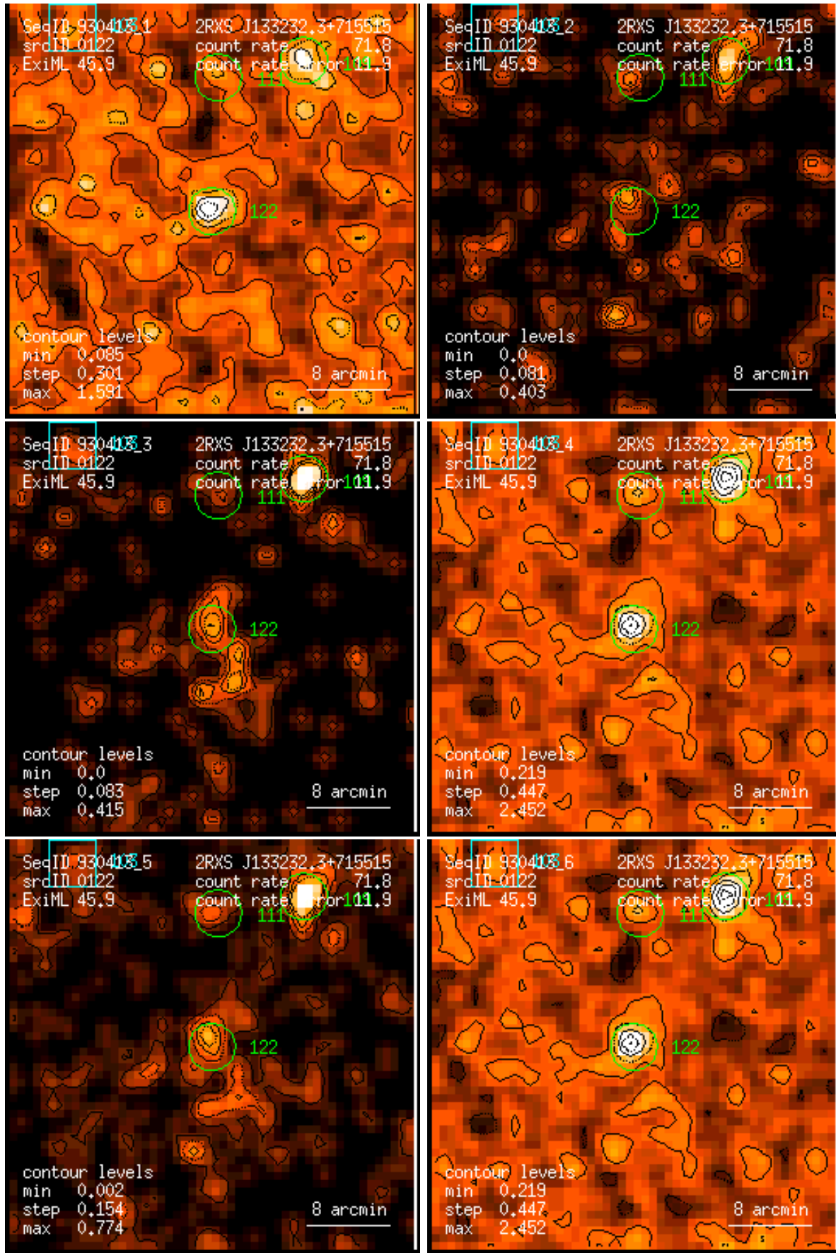
Figure 122: RASS 930413: detection 0122: band rate images, Gaussian filter: (1) PSPC channels 11 – 41, (2) 52 – 90, (3) 91 – 201, (4) 11 – 235, (5) 52 – 201, (6) 11 – 201. Broad band rates in counts/ks. Band rate contour levels in counts/ks/arcmin 2 .
