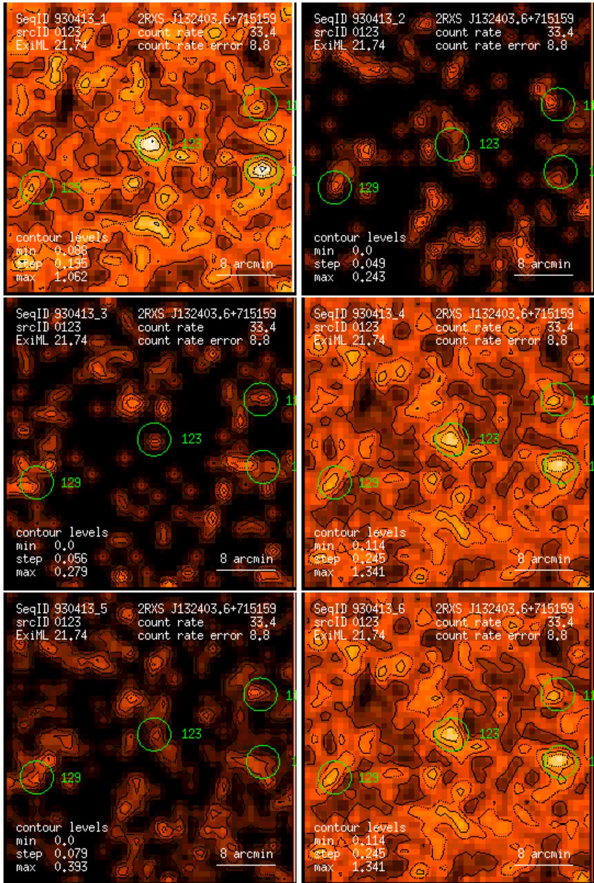
Figure 123: RASS 930413: detection 0123: band rate images, Gaussian filter: (1) PSPPC channels 11 – 41, (2) 52 – 90, (3) 91 – 201, (4) 11 – 235, (5) 52 – 201, (6) 11 – 201. Broad band rates in counts/ks. Band rate contour levels in counts/ks/arcmin 2 .
