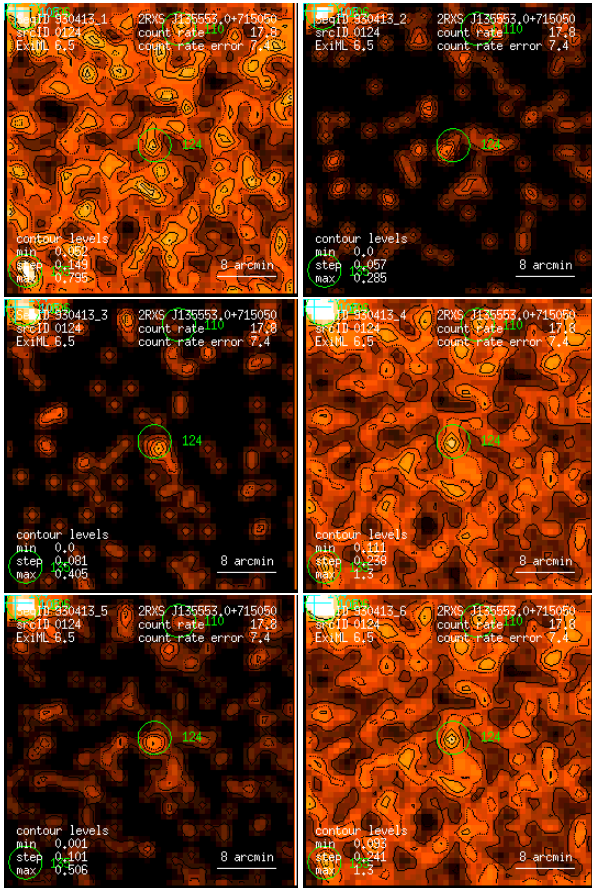
Figure 124: RASS 930413: detection 0124: band rate images, Gaussian filter: (1) PSPC channels 11 – 41, (2) 52 – 90, (3) 91 – 201, (4) 11 – 235, (5) 52 – 201, (6) 11 – 201. Broad band rates in counts/ks. Band rate contour levels in counts/ks/arcmin 2 .
