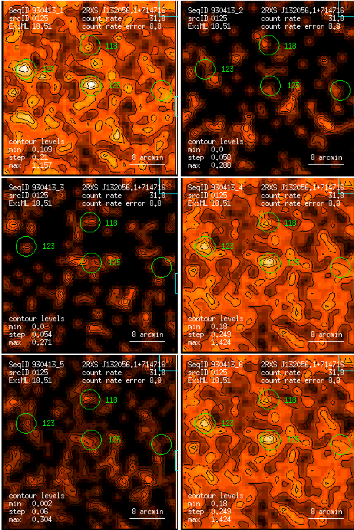
Figure 125: RASS 930413: detection 0125: band rate images, Gaussian filter: (1) PSPC channels 11 – 41, (2) 52 – 90, (3) 91 – 201, (4) 11 – 235, (5) 52 – 201, (6) 11 – 201. Broad band rates in counts/ks. Band rate contour levels in counts/ks/arcmin 2 .
