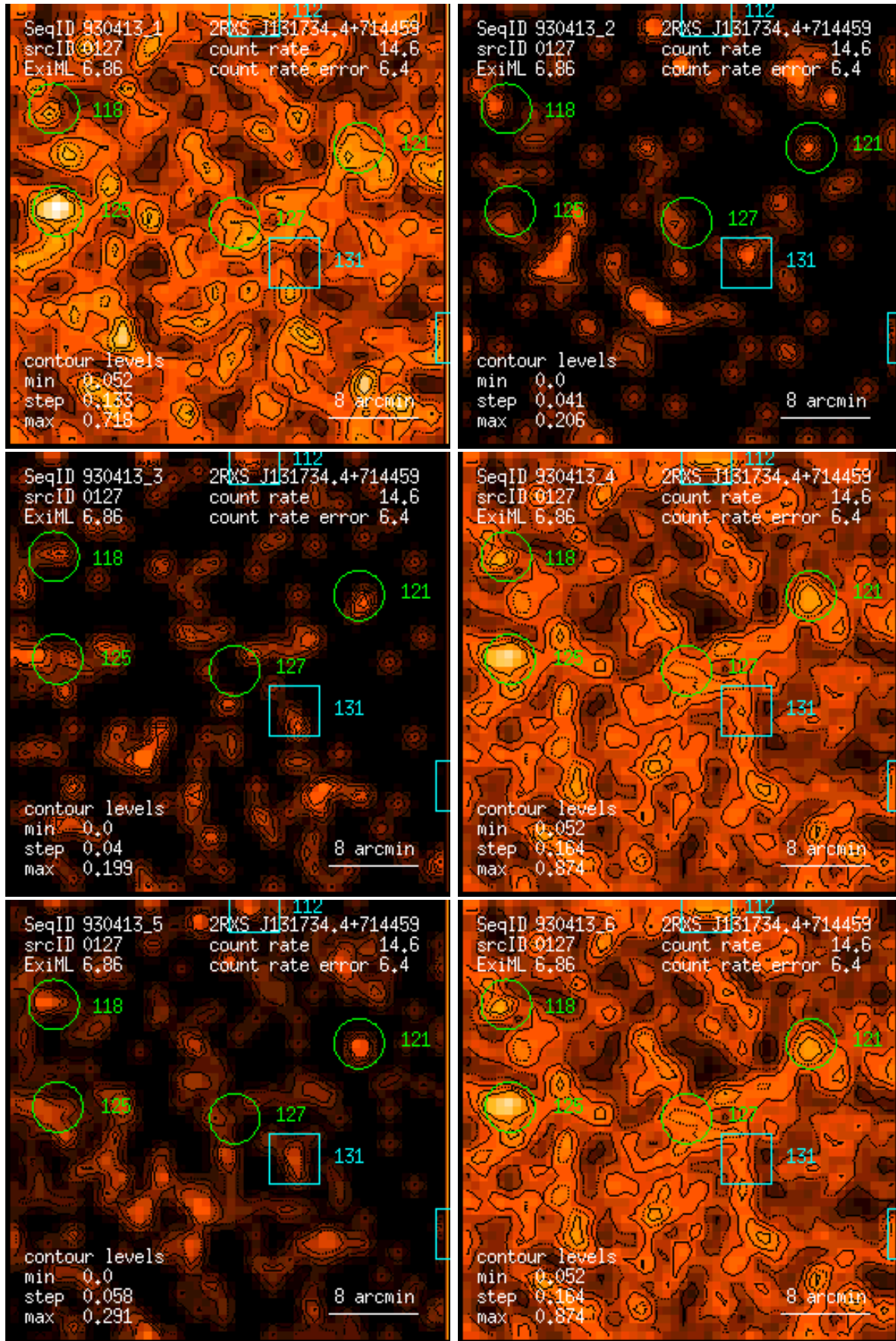
Figure 127: RASS 930413: detection 0127: band rate images, Gaussian filter: (1) PSPC channels 11 – 41, (2) 52 – 90, (3) 91 – 201, (4) 11 – 235, (5) 52 – 201, (6) 11 – 201. Broad band rates in counts/ks. Band rate contour levels in counts/ks/arcmin 2 .
