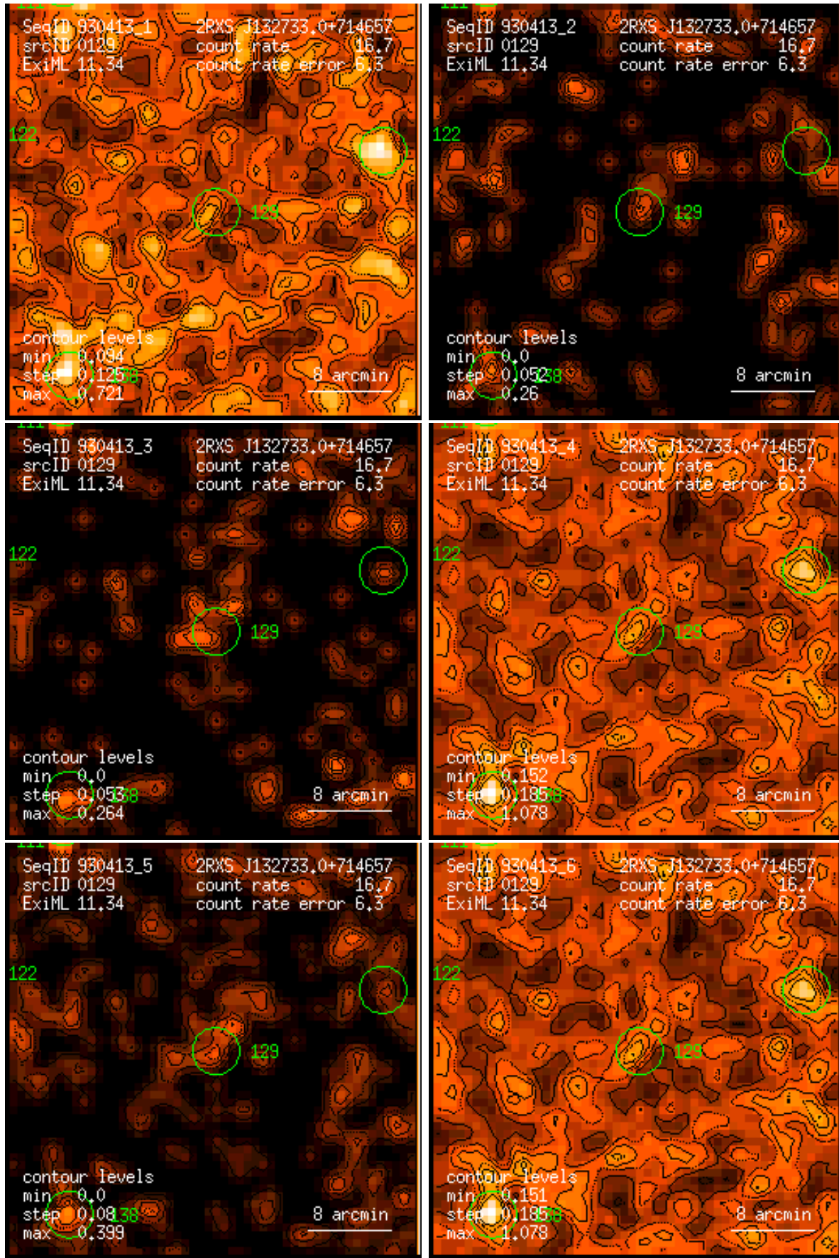
Figure 129: RASS 930413: detection 0129: band rate images, Gaussian filter: (1) PSPC channels 11 – 41, (2) 52 – 90, (3) 91 – 201, (4) 11 – 235, (5) 52 – 201, (6) 11 – 201. Broad band rates in counts/ks. Band rate contour levels in counts/ks/arcmin 2 .
