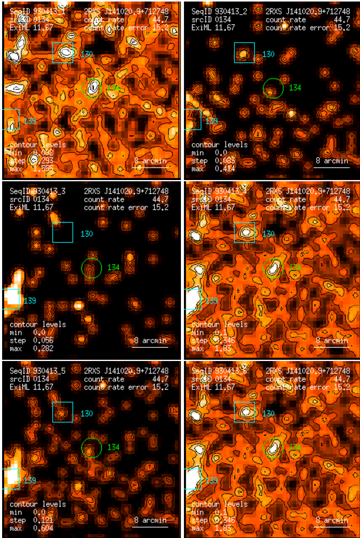
Figure 134: RASS 930413: detection 0134: band rate images, Gaussian filter: (1) PSPC channels 11 – 41, (2) 52 – 90, (3) 91 – 201, (4) 11 – 235, (5) 52 – 201, (6) 11 – 201. Broad band rates in counts/ks. Band rate contour levels in counts/ks/arcmin 2 .
