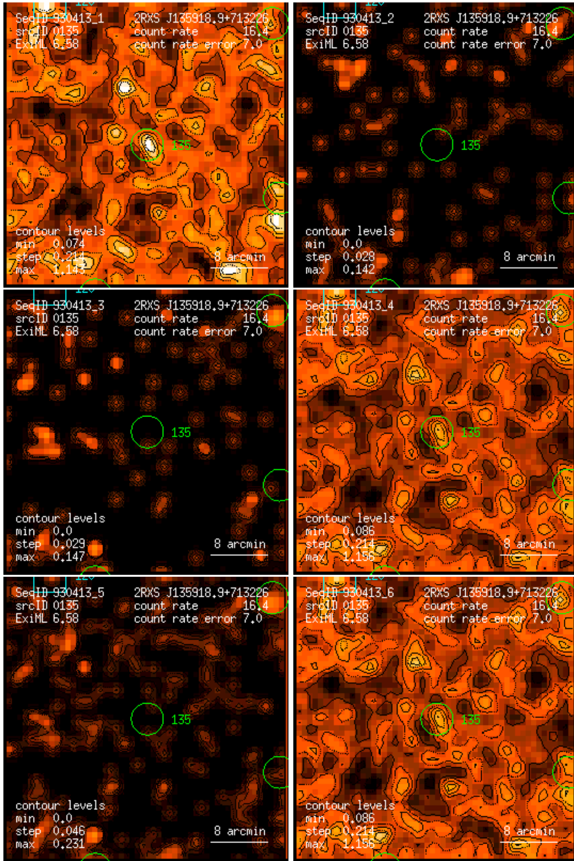
Figure 135: RASS 930413: detection 0135: band rate images, Gaussian filter: (1) PSPC channels 11 – 41, (2) 52 – 90, (3) 91 – 201, (4) 11 – 235, (5) 52 – 201, (6) 11 – 201. Broad band rates in counts/ks. Band rate contour levels in counts/ks/arcmin 2 .
