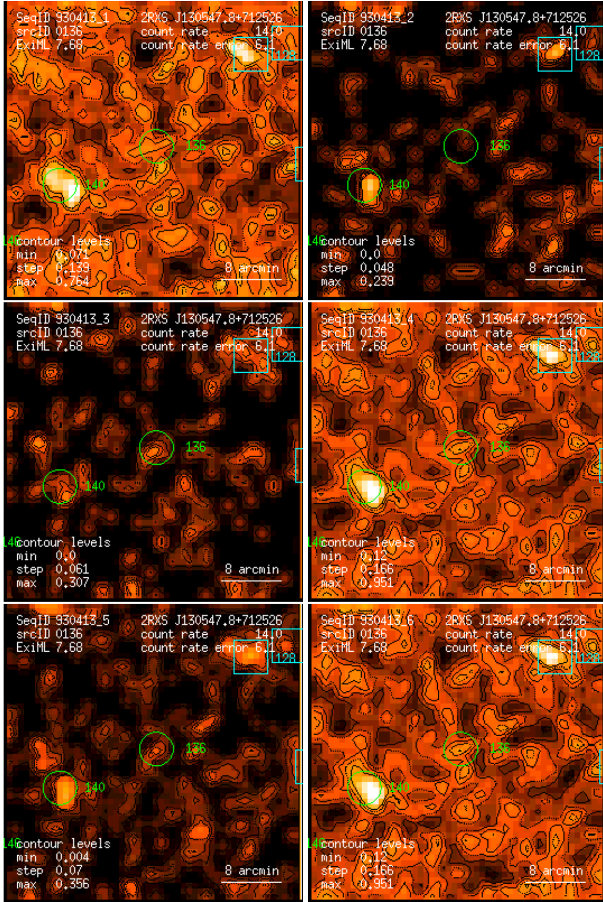
Figure 136: RASS 930413: detection 0136: band rate images, Gaussian filter: (1) PSPC channels 11 – 41, (2) 52 – 90, (3) 91 – 201, (4) 11 – 235, (5) 52 – 201, (6) 11 – 201. Broad band rates in counts/ks. Band rate contour levels in counts/ks/arcmin 2 .
