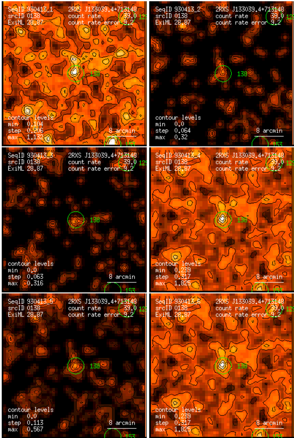
Figure 138: RASS 930413: detection 0138: band rate images, Gaussian filter: (1) PSPC channels 11 – 41, (2) 52 – 90, (3) 91 – 201, (4) 11 – 235, (5) 52 – 201, (6) 11 – 201. Broad band rates in counts/ks. Band rate contour levels in counts/ks/arcmin 2 .
