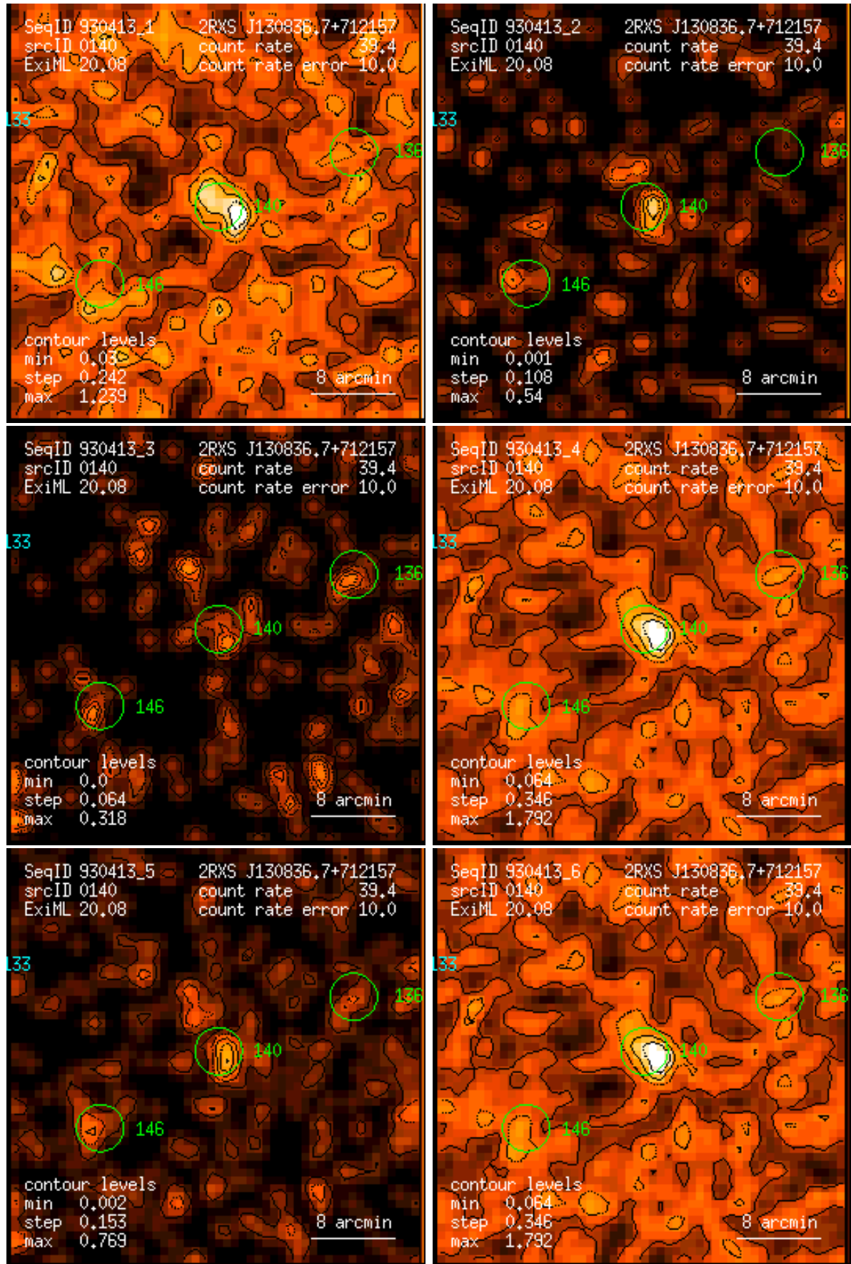
Figure 140: RASS 930413: detection 0140: band rate images, Gaussian filter: (1) PSPC channels 11 – 41, (2) 52 – 90, (3) 91 – 201, (4) 11 – 235, (5) 52 – 201, (6) 11 – 201. Broad band rates in counts/ks. Band rate contour levels in counts/ks/arcmin 2 .
