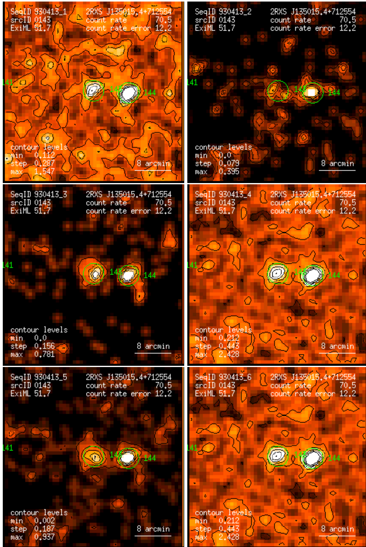
Figure 143: RASS 930413: detection 0143: band rate images, Gaussian filter: (1) PSPC channels 11 – 41, (2) 52 – 90, (3) 91 – 201, (4) 11 – 235, (5) 52 – 201, (6) 11 – 201. Broad band rates in counts/ks. Band rate contour levels in counts/ks/arcmin 2 .
