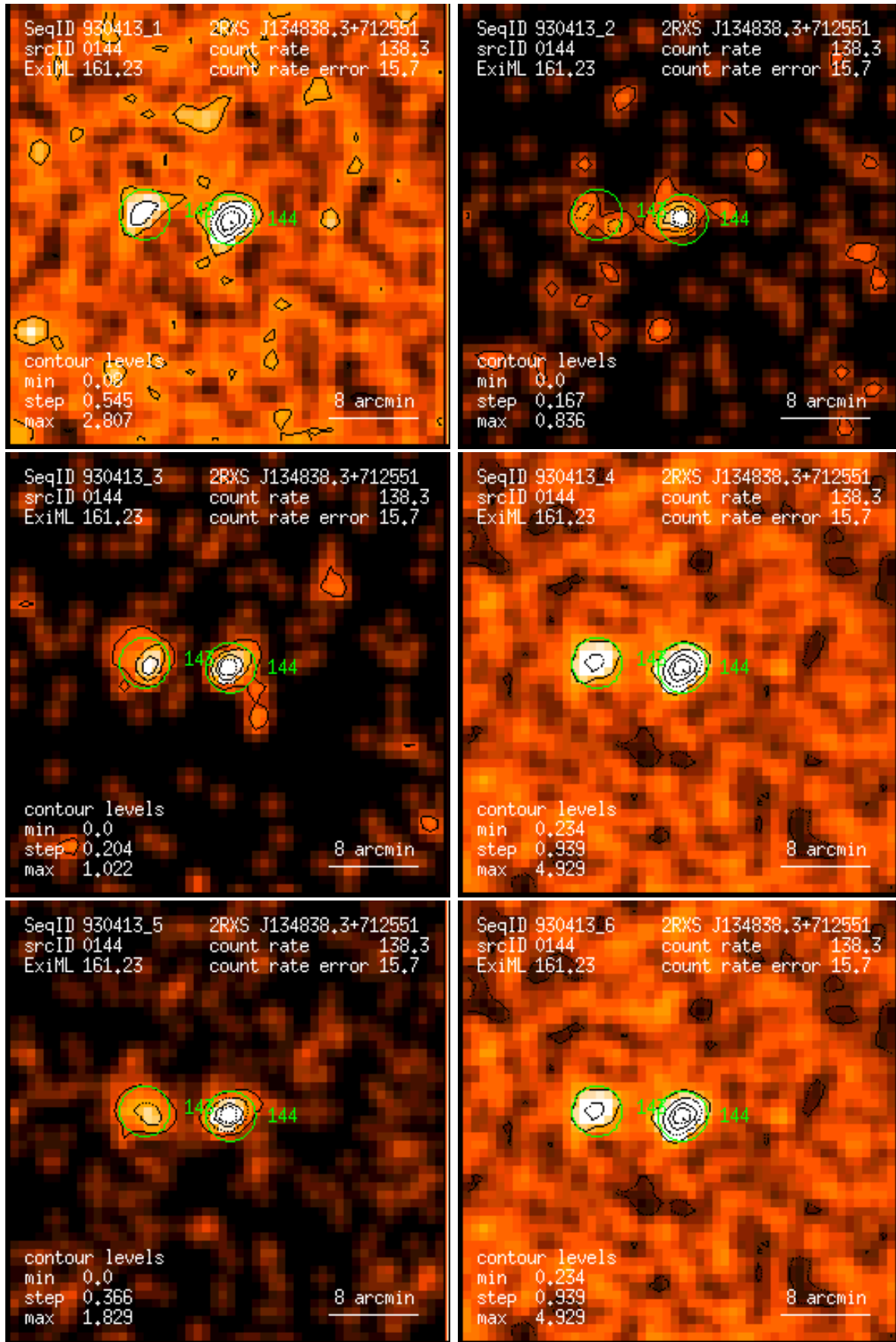
Figure 144: RASS 930413: detection 0144: band rate images, Gaussian filter: (1) PSPC channels 11 – 41, (2) 52 – 90, (3) 91 – 201, (4) 11 – 235, (5) 52 – 201, (6) 11 – 201. Broad band rates in counts/ks. Band rate contour levels in counts/ks/arcmin 2 .
