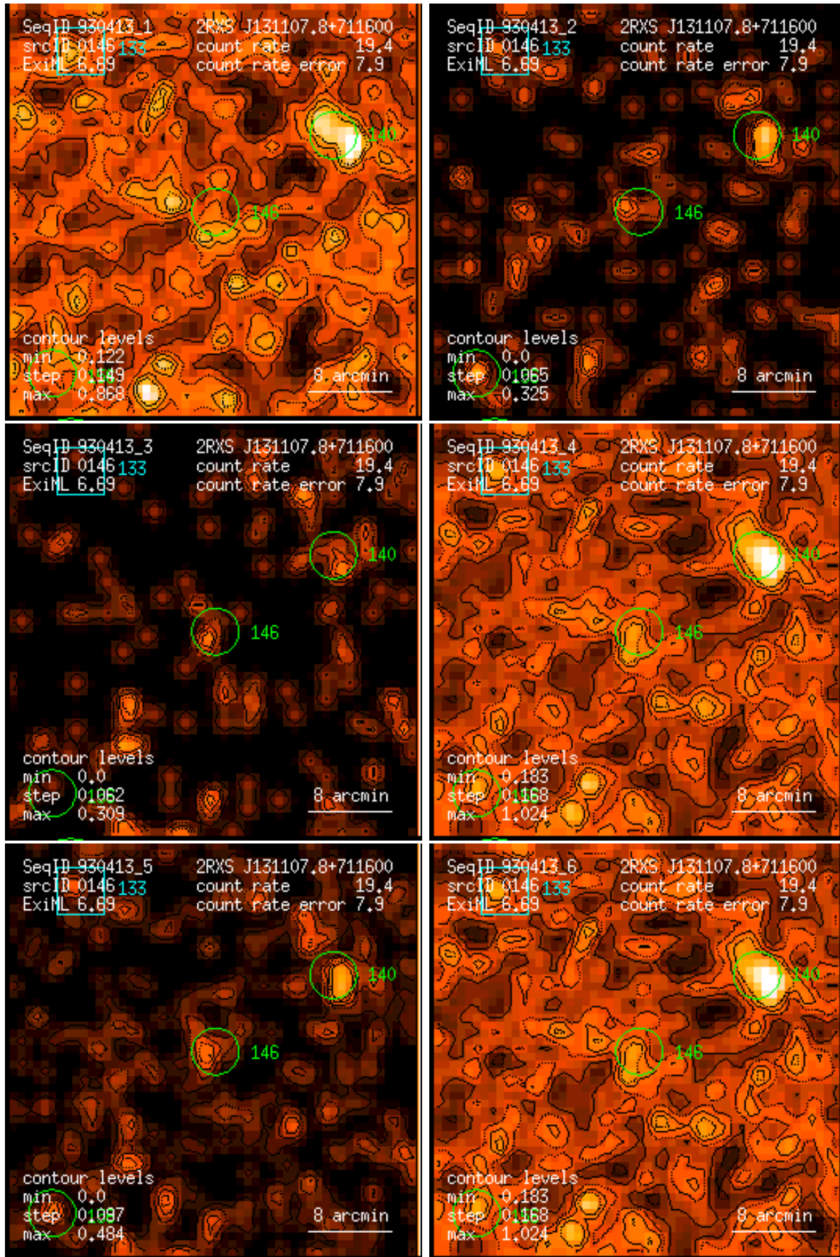
Figure 146: RASS 930413: detection 0146: band rate images, Gaussian filter: (1) PSPC channels 11 – 41, (2) 52 – 90, (3) 91 – 201, (4) 11 – 235, (5) 52 – 201, (6) 11 – 201. Broad band rates in counts/ks. Band rate contour levels in counts/ks/arcmin 2 .
