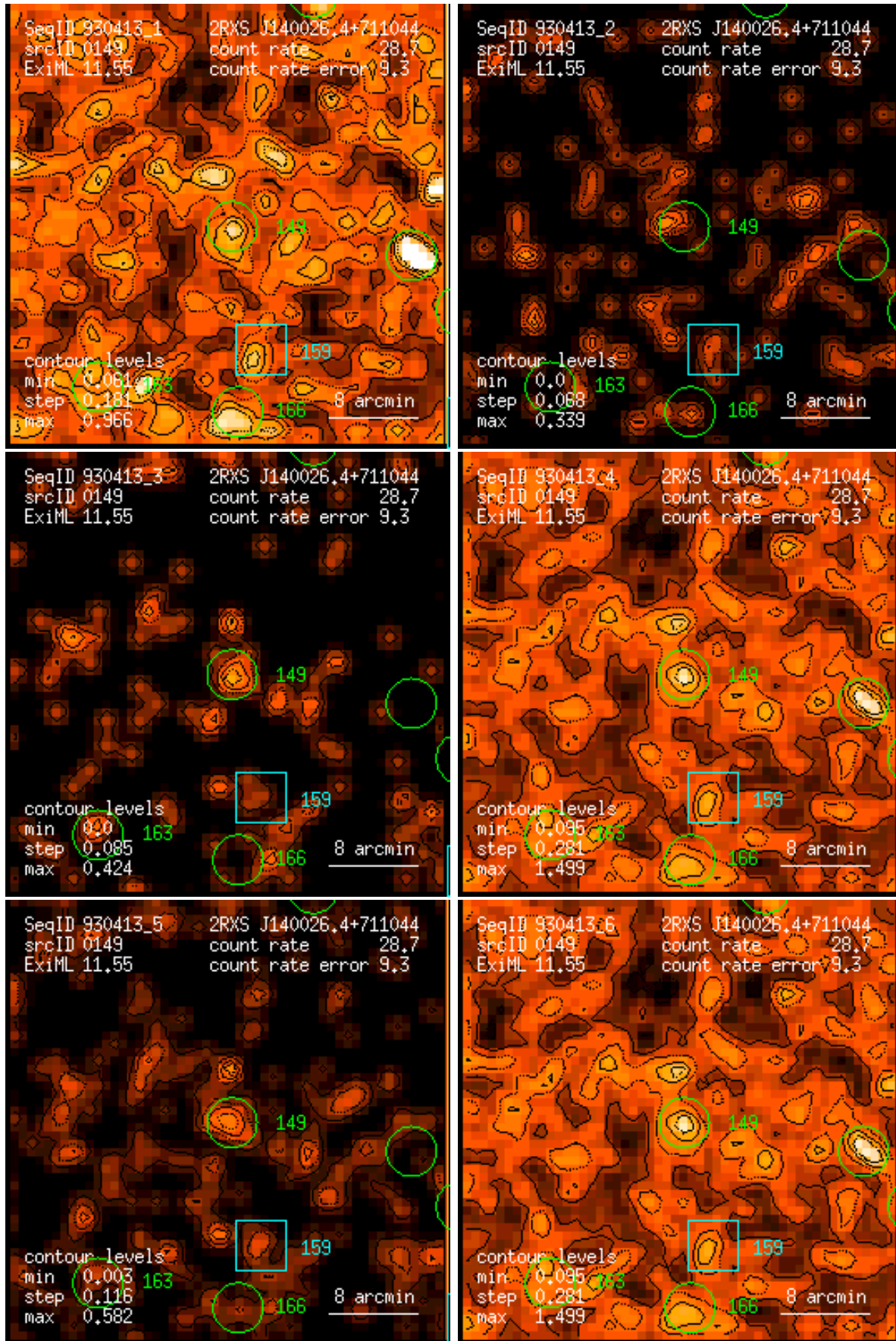
Figure 149: RASS 930413: detection 0149: band rate images, Gaussian filter: (1) PSPC channels 11 – 41, (2) 52 – 90, (3) 91 – 201, (4) 11 – 235, (5) 52 – 201, (6) 11 – 201. Broad band rates in counts/ks. Band rate contour levels in counts/ks/arcmin 2 .
