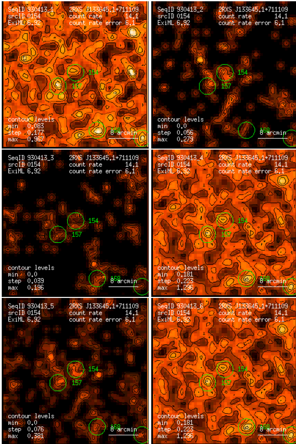
Figure 154: RASS 930413: detection 0154: band rate images, Gaussian filter: (1) PSPC channels 11 – 41, (2) 52 – 90, (3) 91 – 201, (4) 11 – 235, (5) 52 – 201, (6) 11 – 201. Broad band rates in counts/ks. Band rate contour levels in counts/ks/arcmin 2 .
