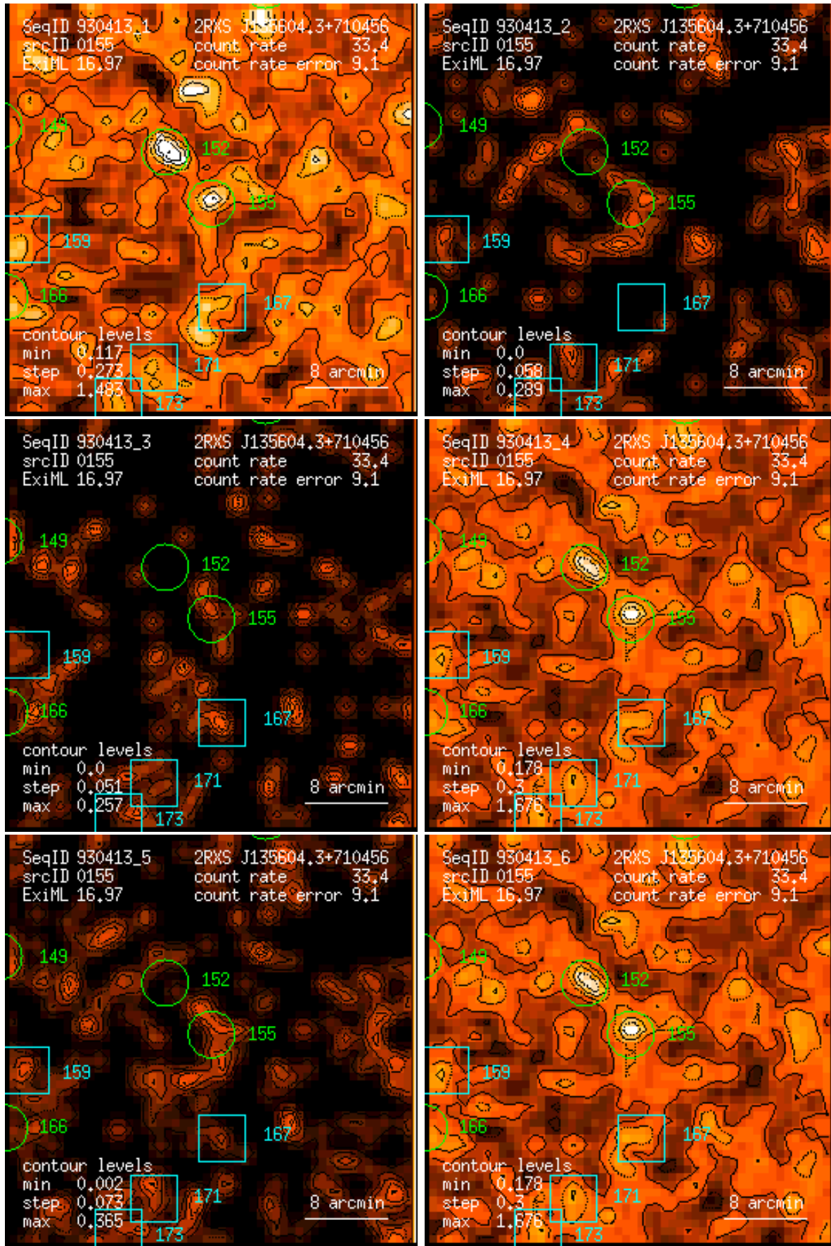
Figure 155: RASS 930413: detection 0155: band rate images, Gaussian filter: (1) PSPC channels 11 – 41, (2) 52 – 90, (3) 91 – 201, (4) 11 – 235, (5) 52 – 201, (6) 11 – 201. Broad band rates in counts/ks. Band rate contour levels in counts/ks/arcmin 2 .
