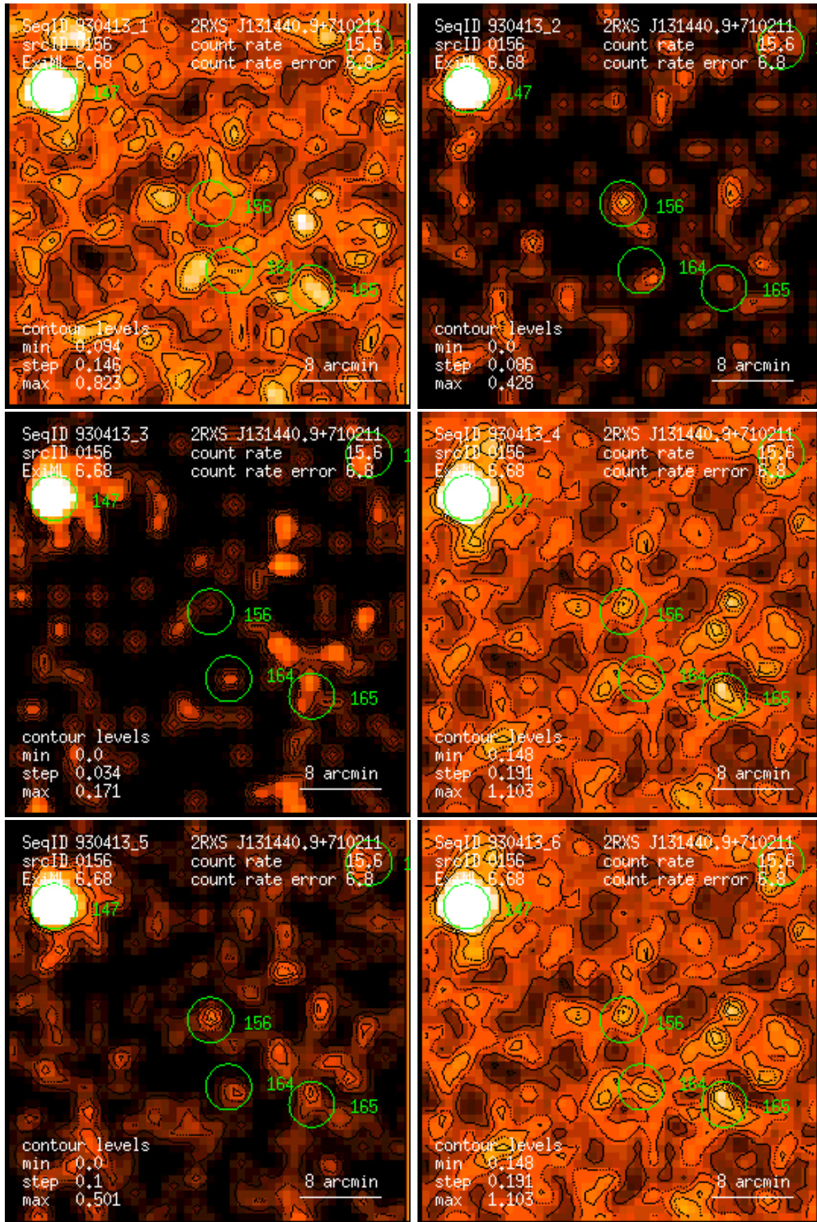
Figure 156: RASS 930413: detection 0156: band rate images, Gaussian filter: (1) PSPC channels 11 – 41, (2) 52 – 90, (3) 91 – 201, (4) 11 – 235, (5) 52 – 201, (6) 11 – 201. Broad band rates in counts/ks. Band rate contour levels in counts/ks/arcmin 2 .
